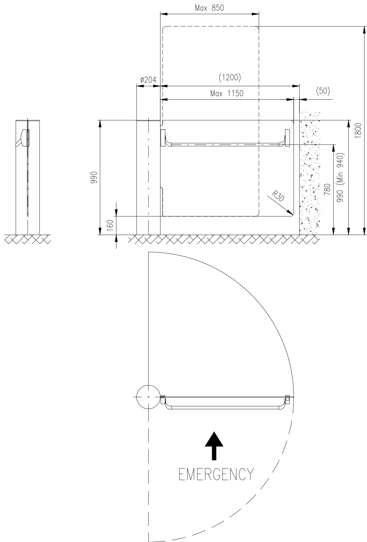
Motorized gate: PEGAS–HG–204–Right–Emergency
