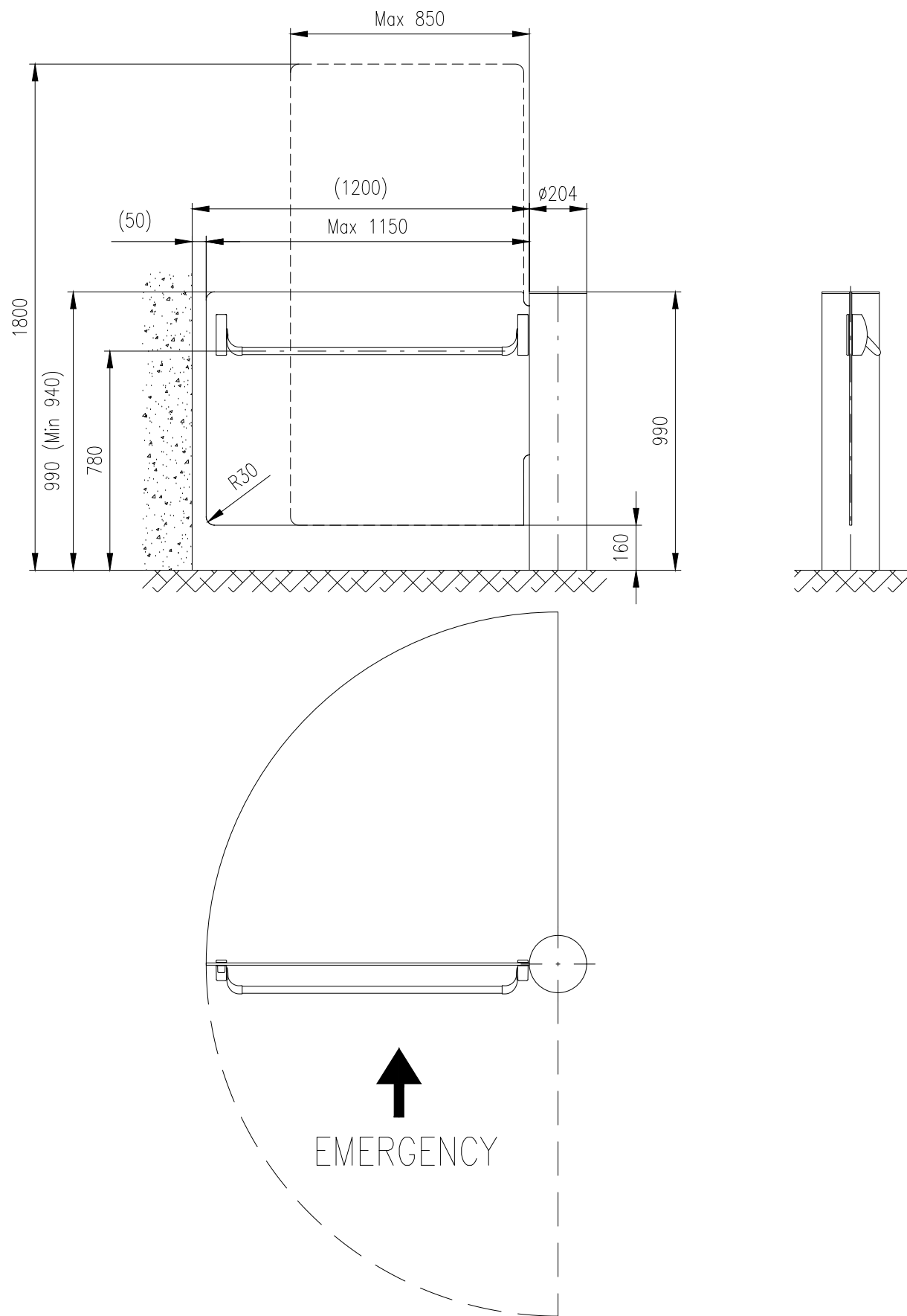
Motorized gate: PEGAS–HG–204–Left–Emergency
