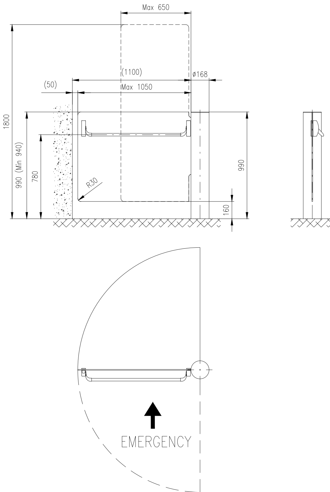
Motorized gate: PEGAS–GLE–168–Left–Emergency
