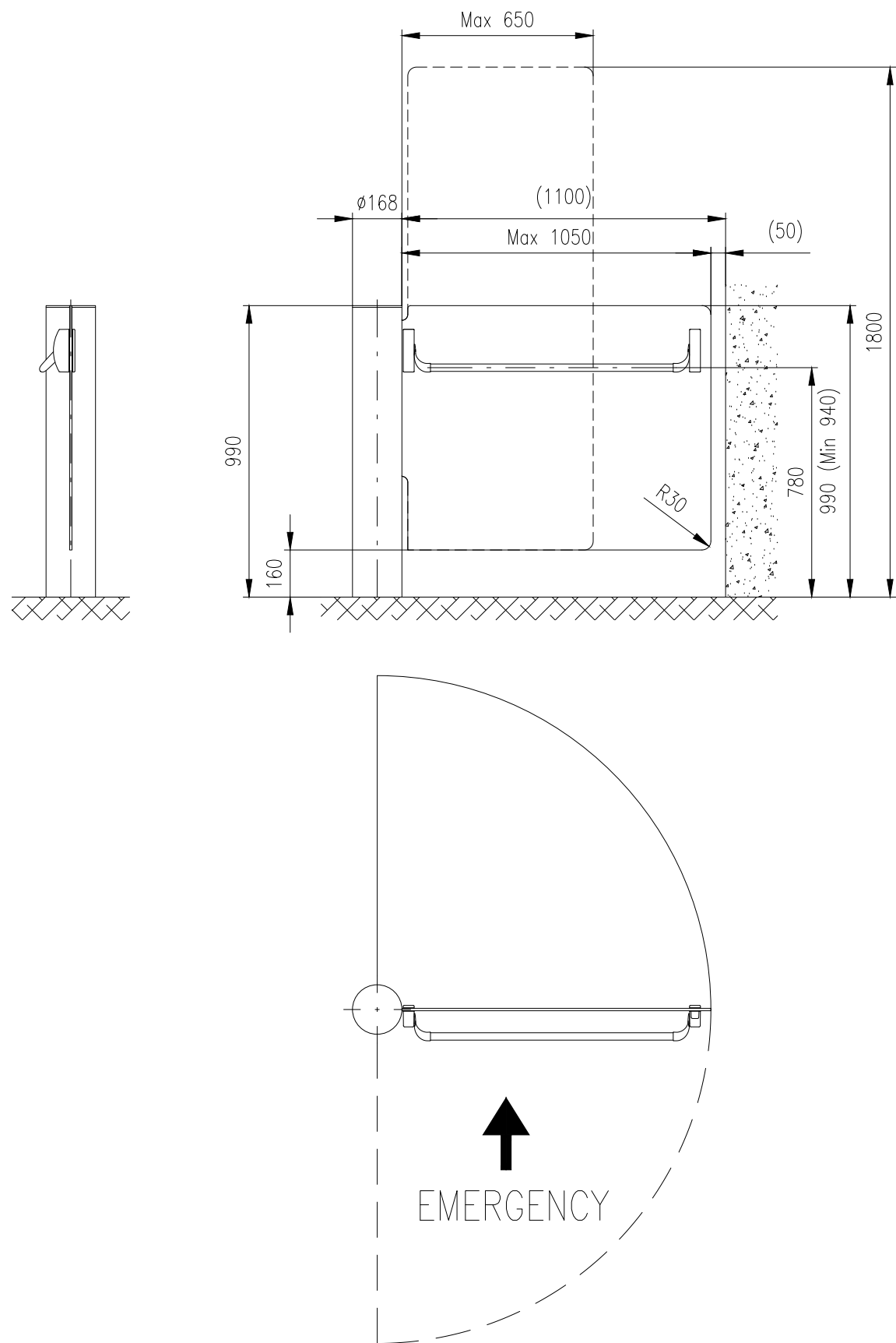
Motorized gate: PEGAS–GLE–168–Right–Emergency
