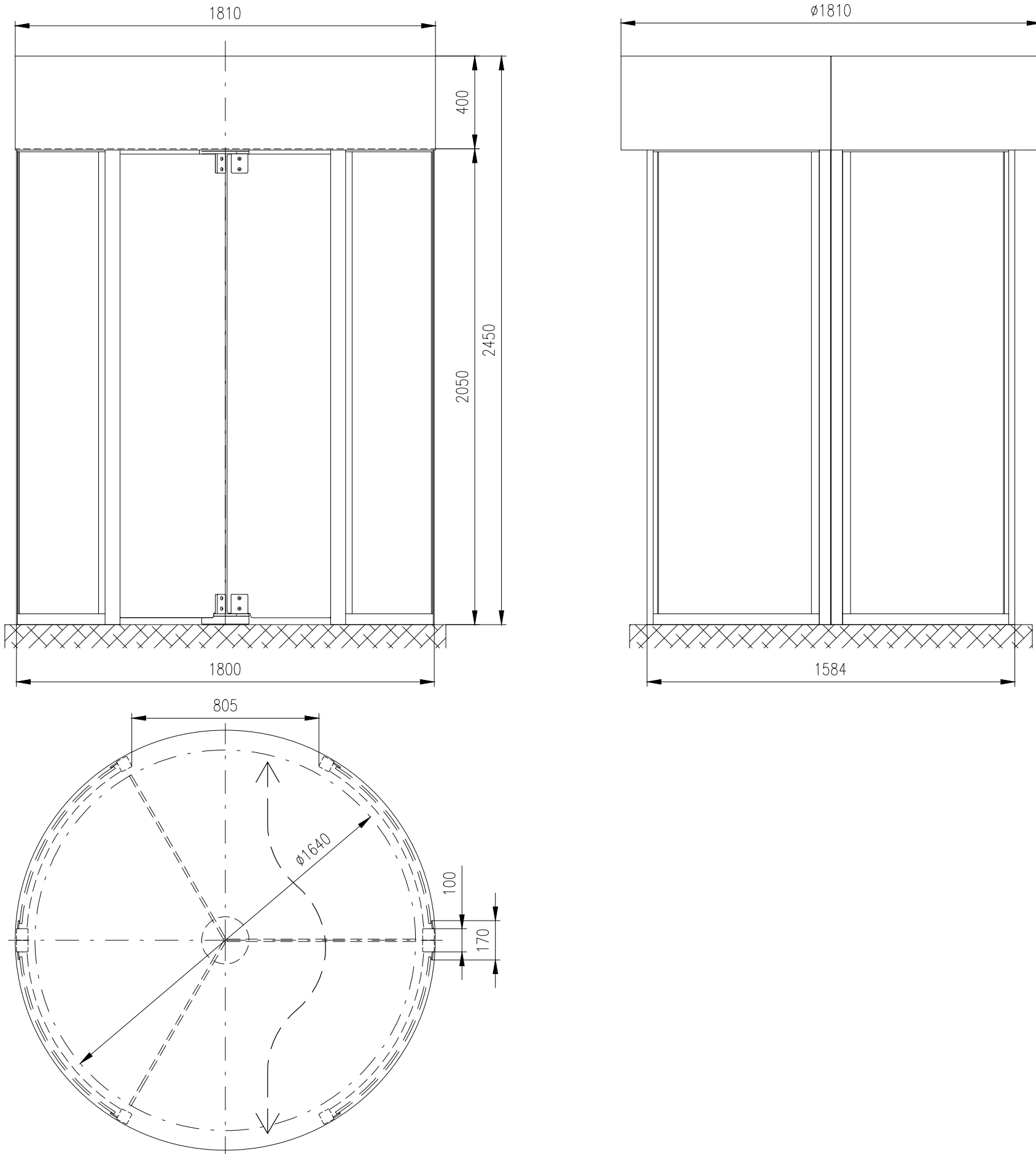
Motorized turnstile: REXON-DEA-GLASS (1800)
