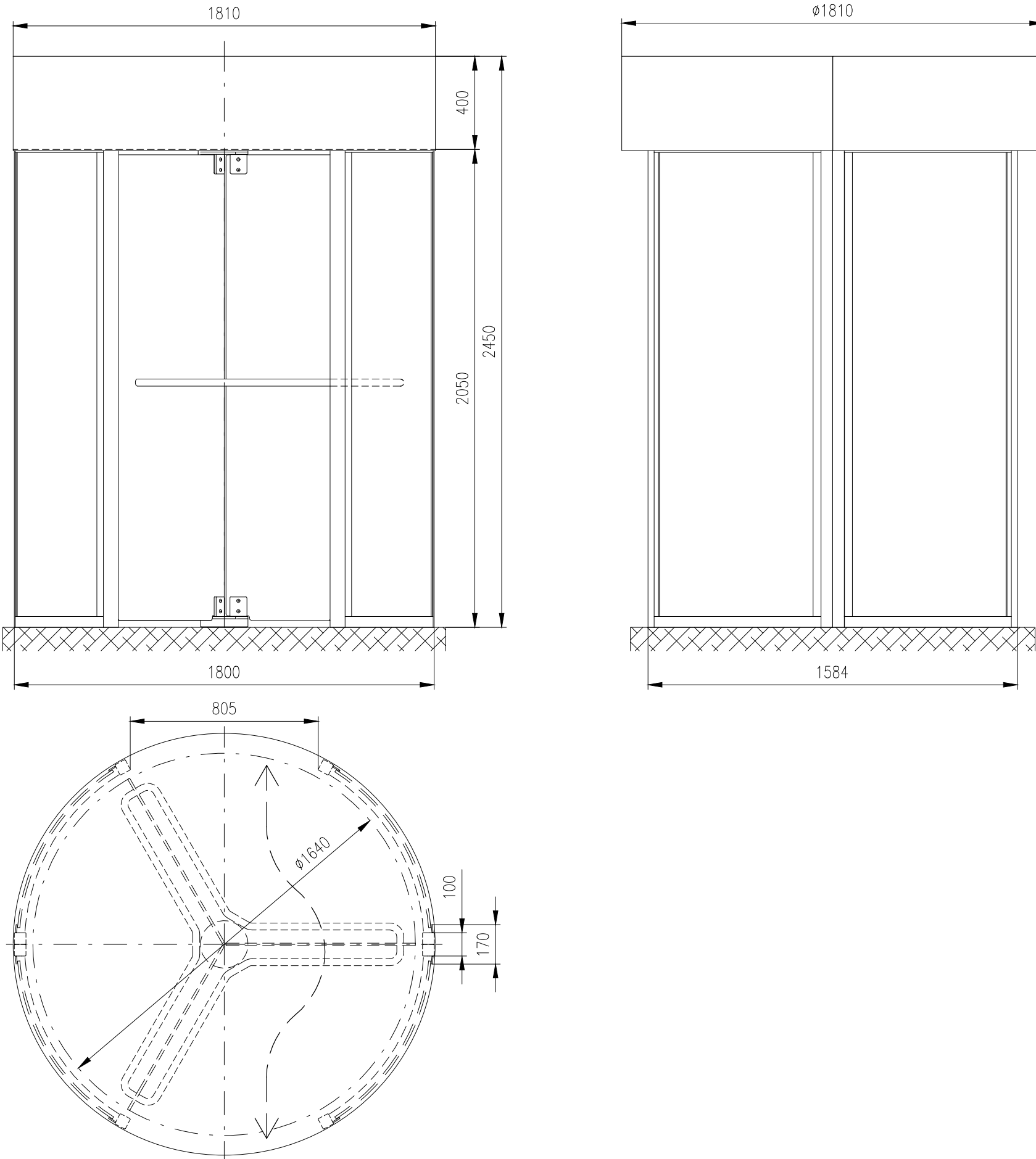
Motorized turnstile: REXON-DEA-GLASS (1800) (with push bar)
