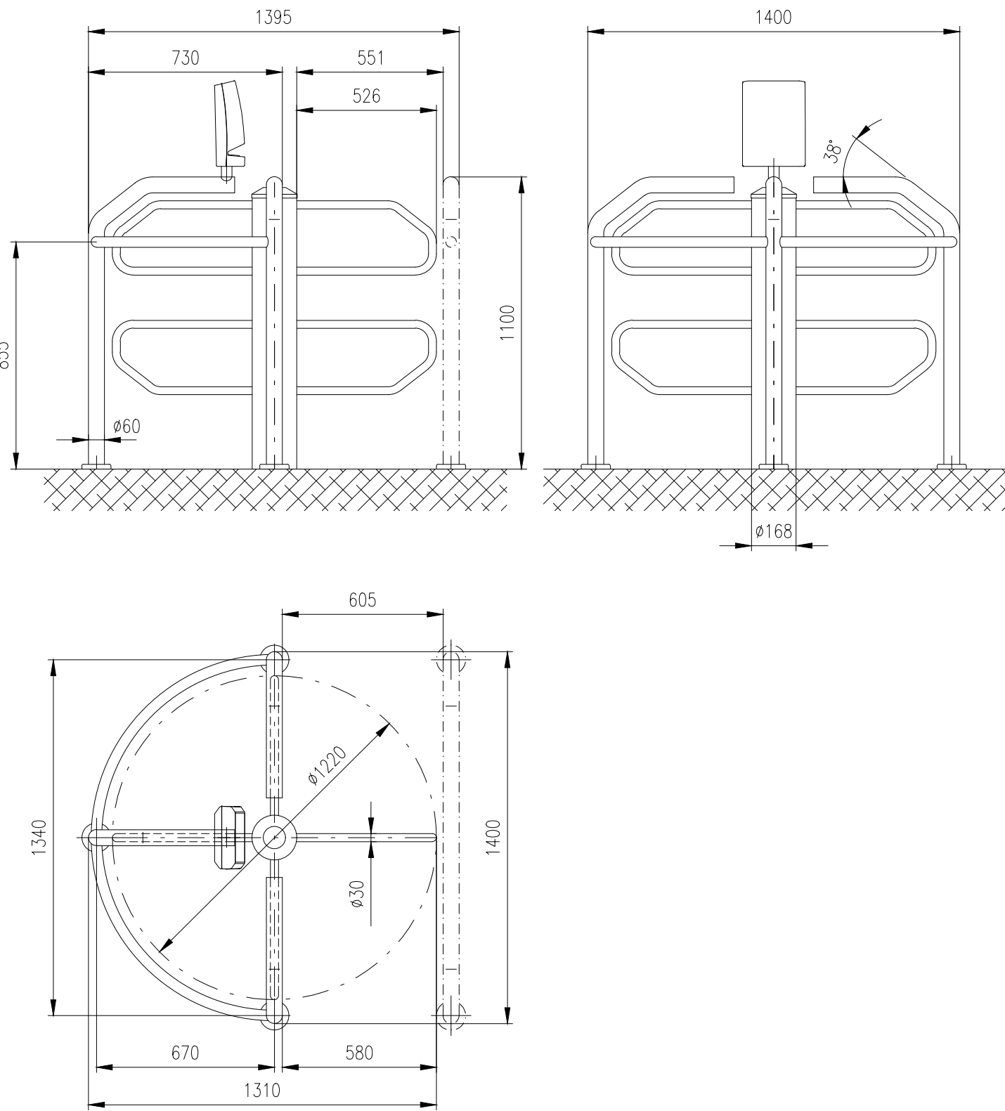
Motorized turnstile: ROUND-J-90-U-168 (1220)
