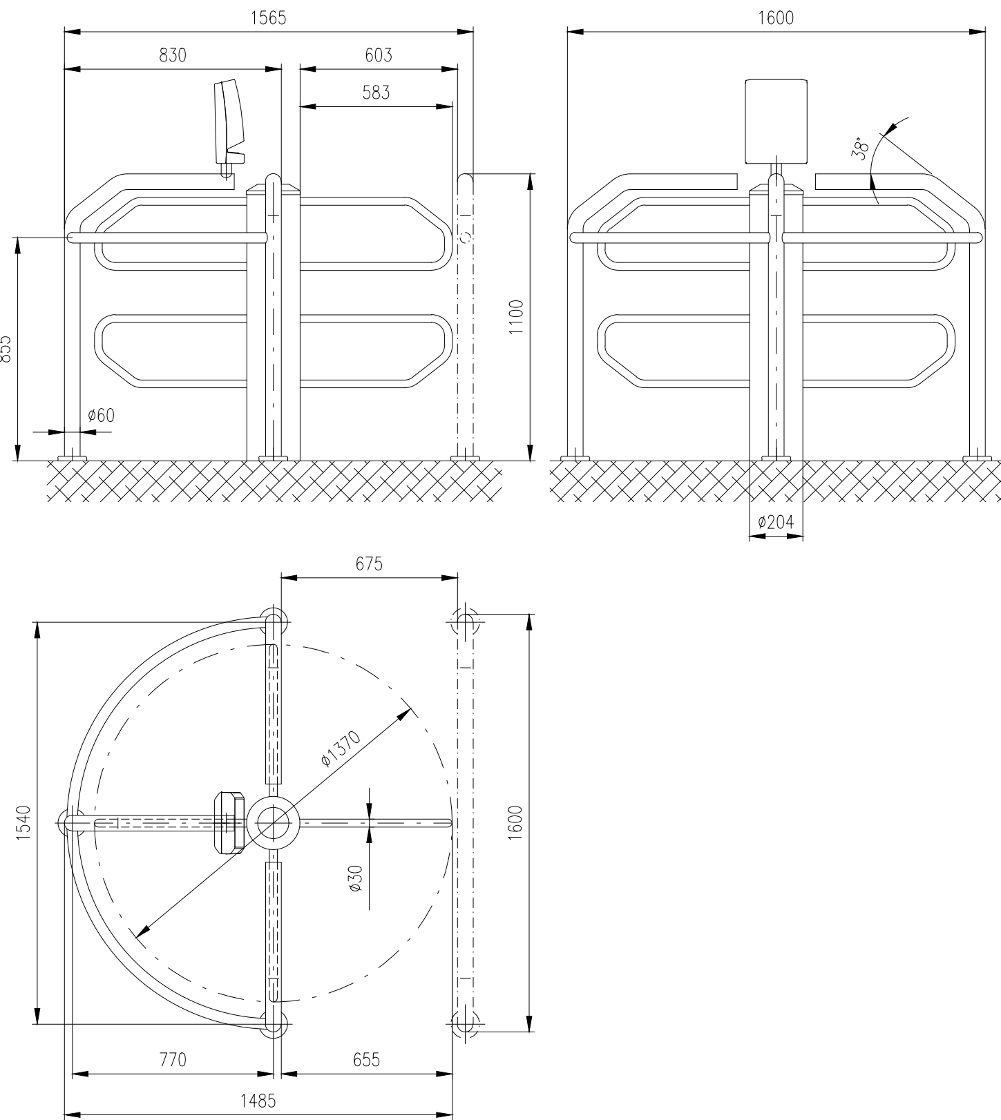
Motorized turnstile: ROUND-J-90-U-204 (1370)
