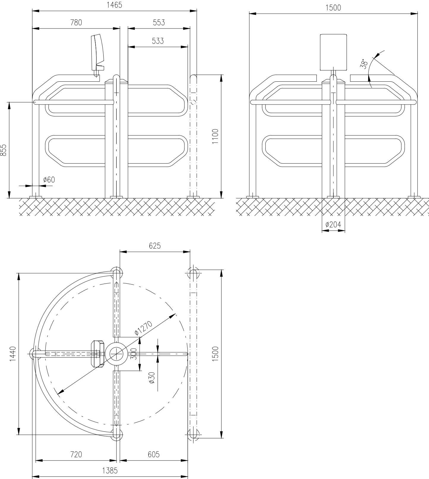
Motorized turnstile: ROUND-J-90-U-204 (1270)
