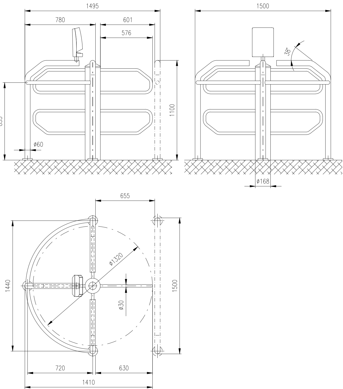
Motorized turnstile: ROUND-J-90-U-168 (1320)
