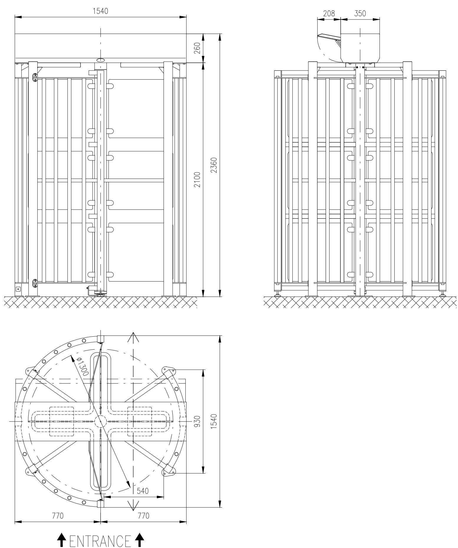
Motorized turnstile: REXON-ERA-4-FULL-G
