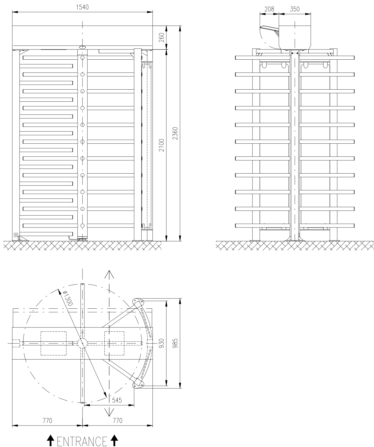
Motorized turnstile: REXON-ERA-4-GS
