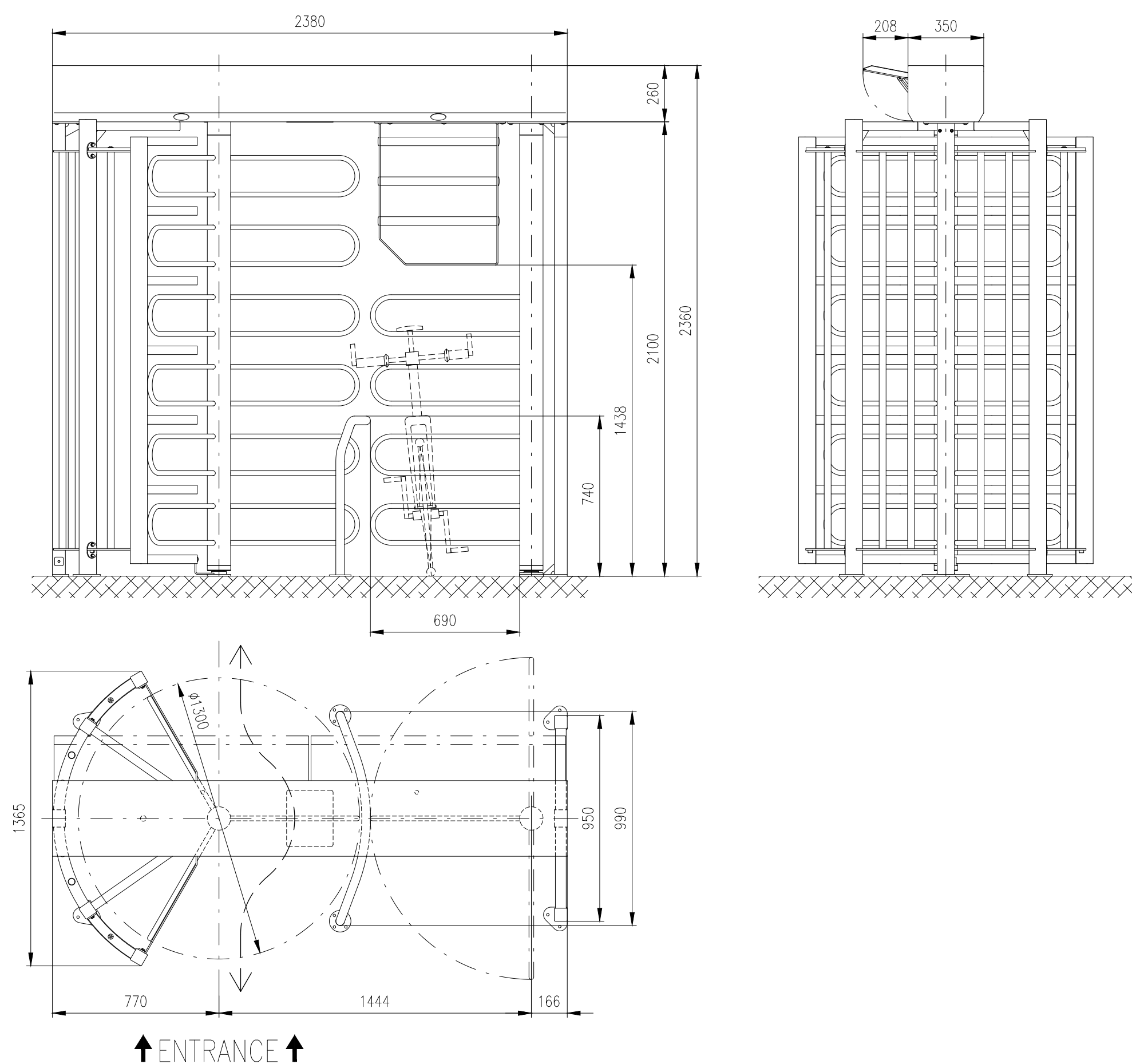
Motorized turnstile: REXON-ERA-3-BIKE-U
