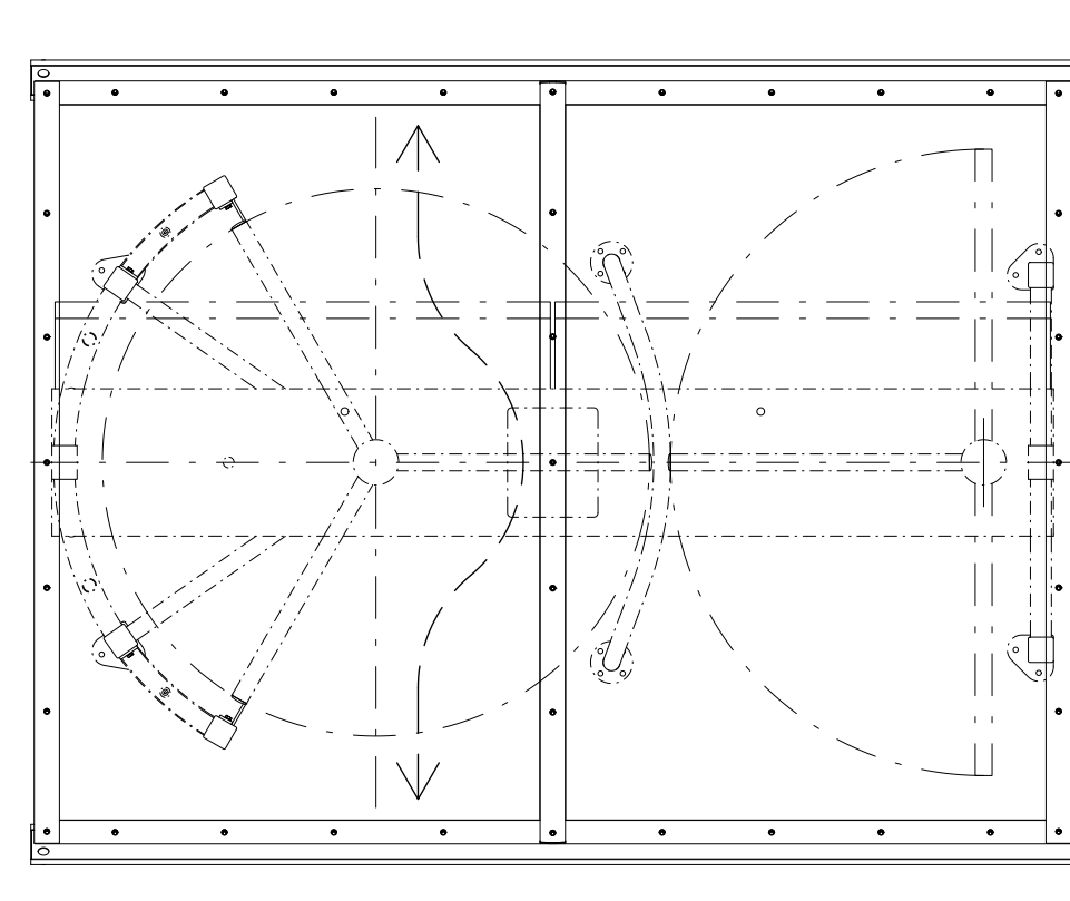
Roof for turnstile: REXON-ERA-BIKE
