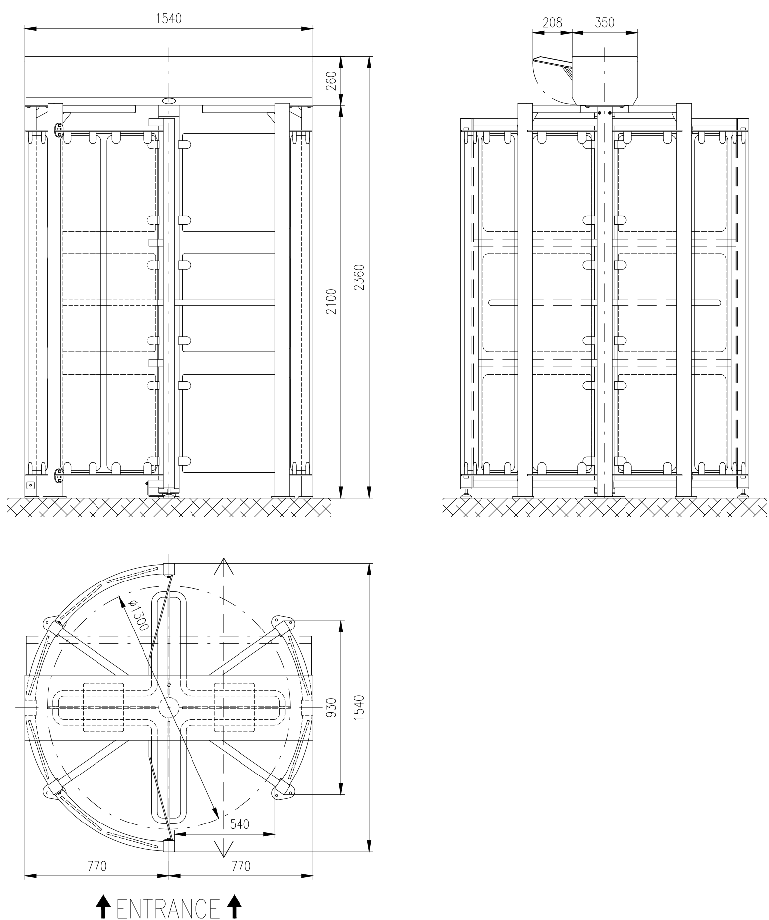
Motorized turnstile: REXON-ERA-4-FULL-GS-G
