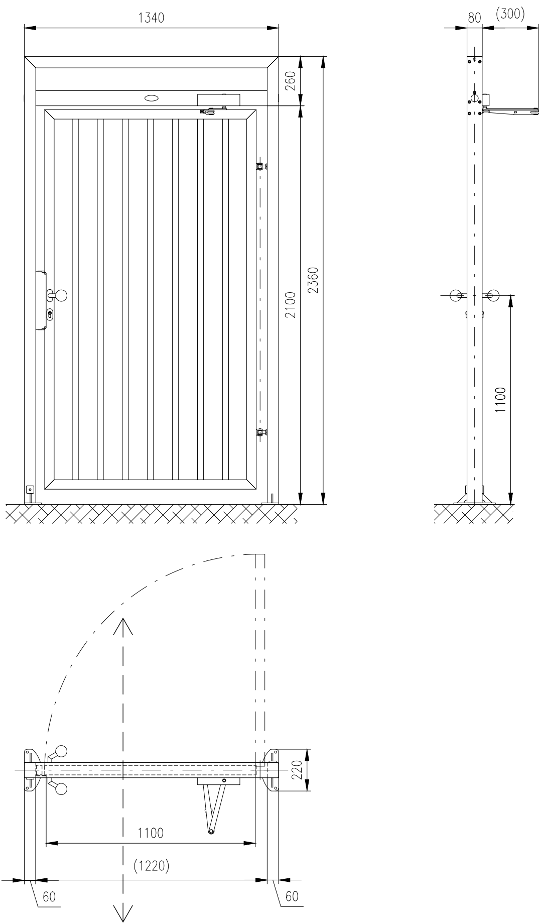
PedGate: Left-Hand (electric lock)
