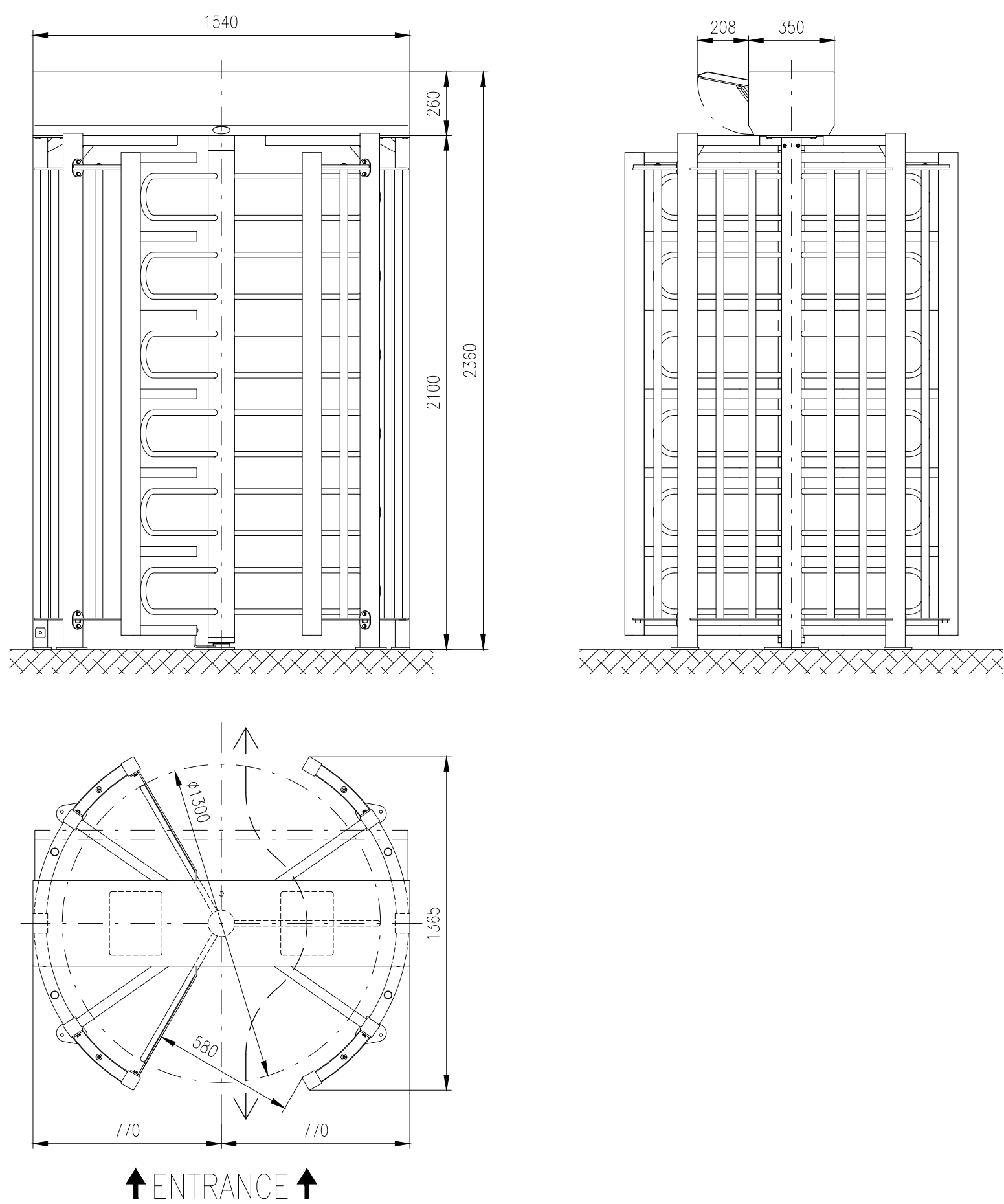
Motorized turnstile: REXON-ERA-3-FULL-U
