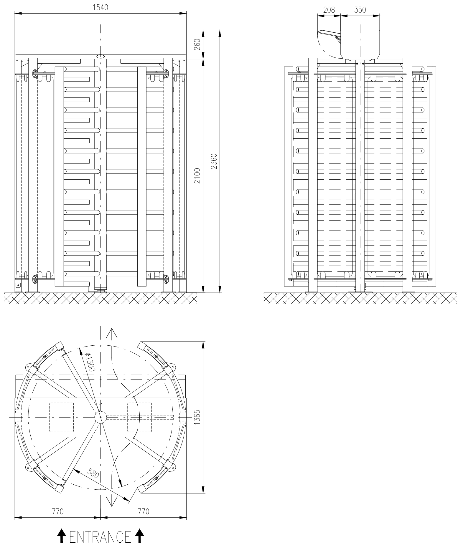
Motorized turnstile: REXON-ERA-4-FULL-GS
