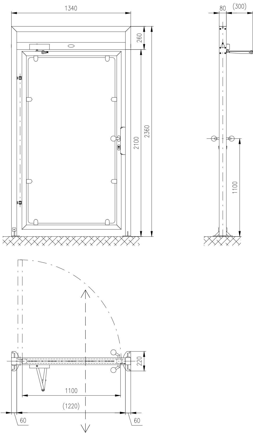
PedGate-GS: Left-Hand (electric lock)
