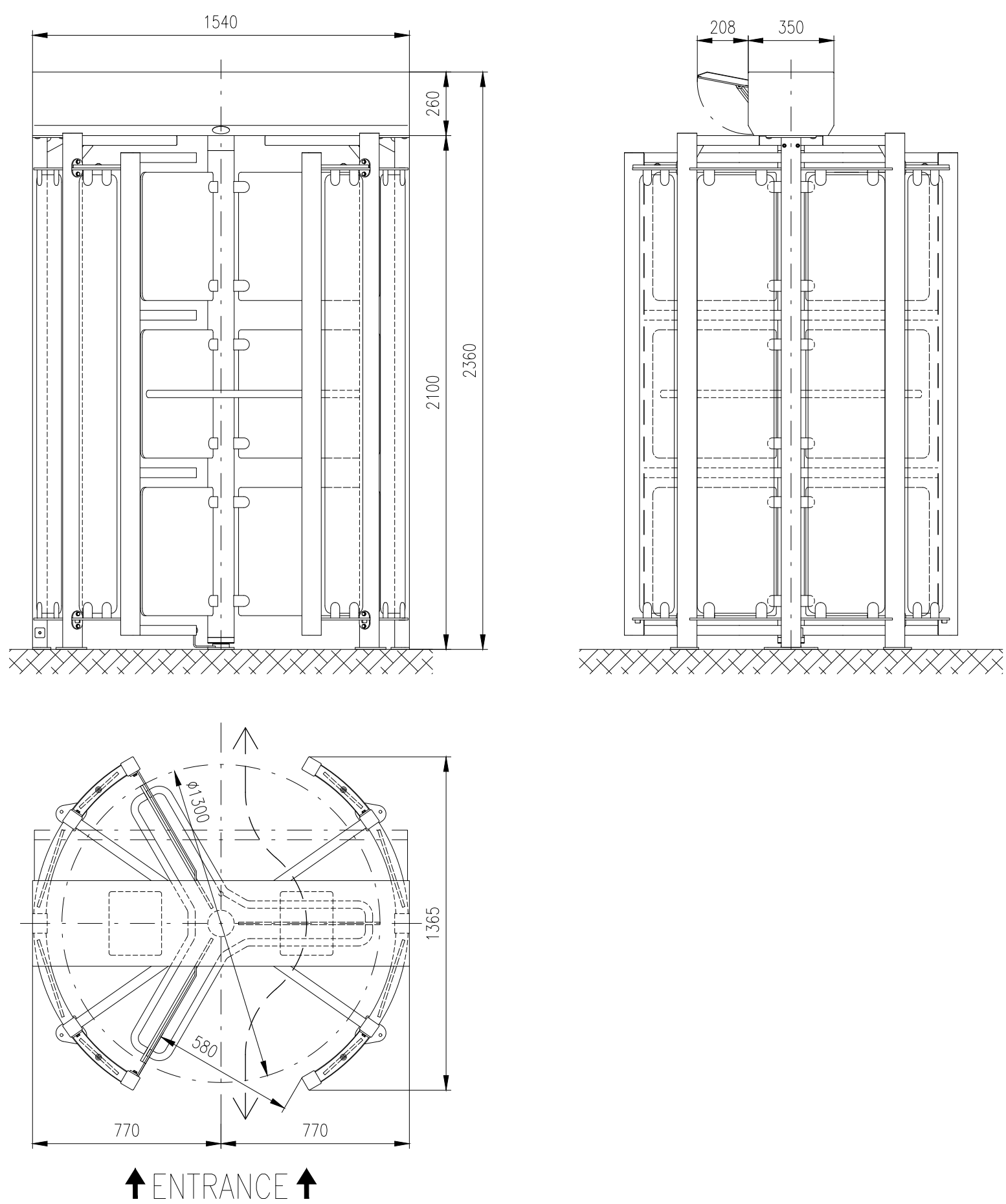
Motorized turnstile: REXON-ERA-3-FULL-GS-G
