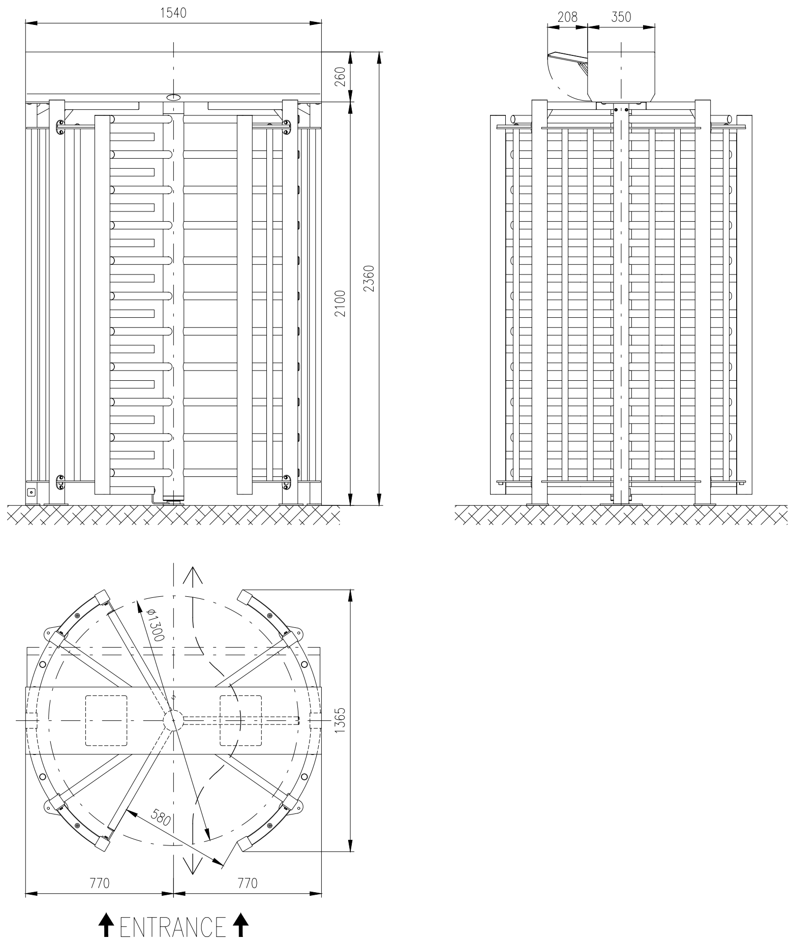
Motorized turnstile: REXON-ERA-4-FULL
