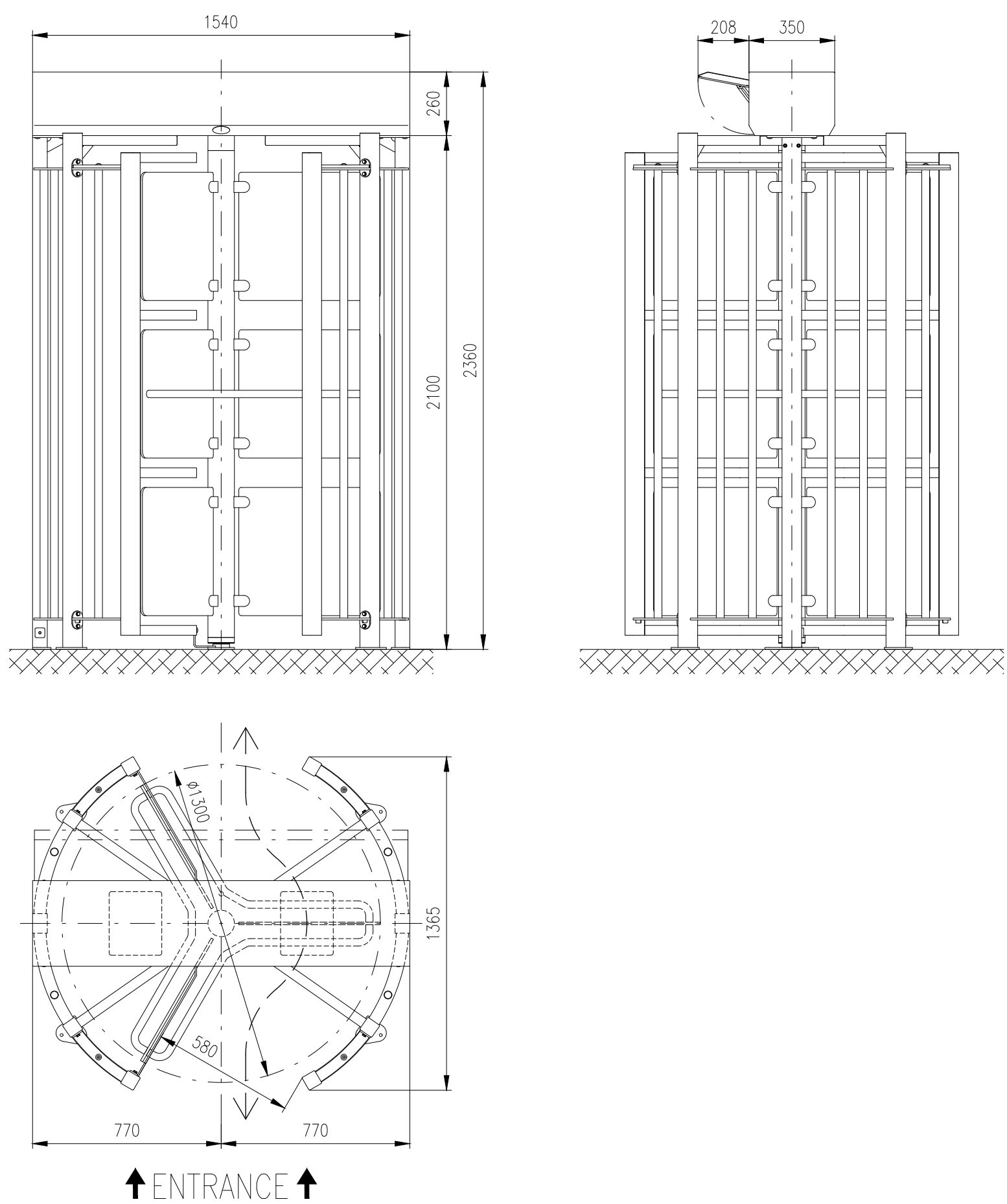
Motorized turnstile: REXON-ERA-3-FULL-G
