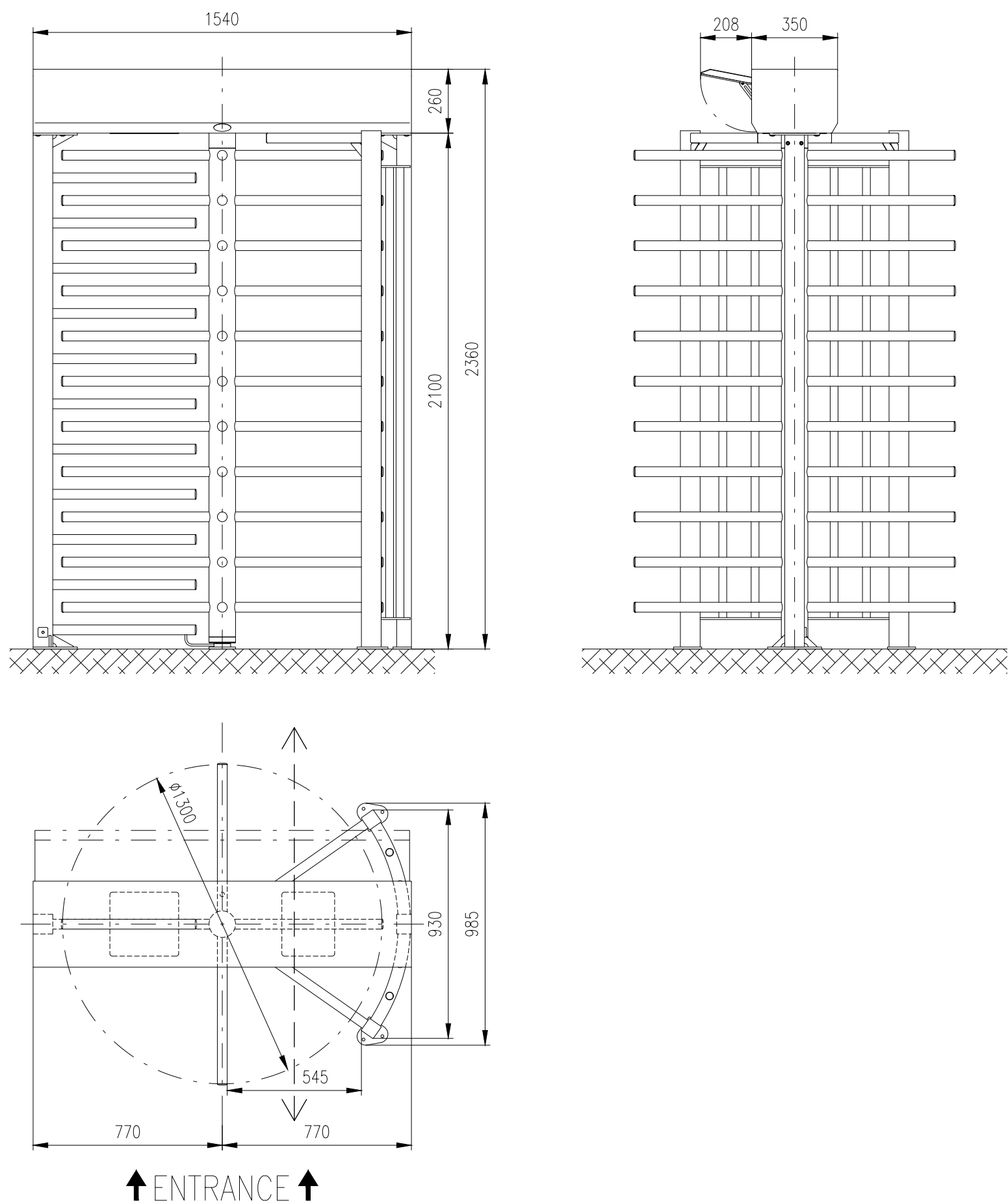
Motorized turnstile: REXON-ERA-4
