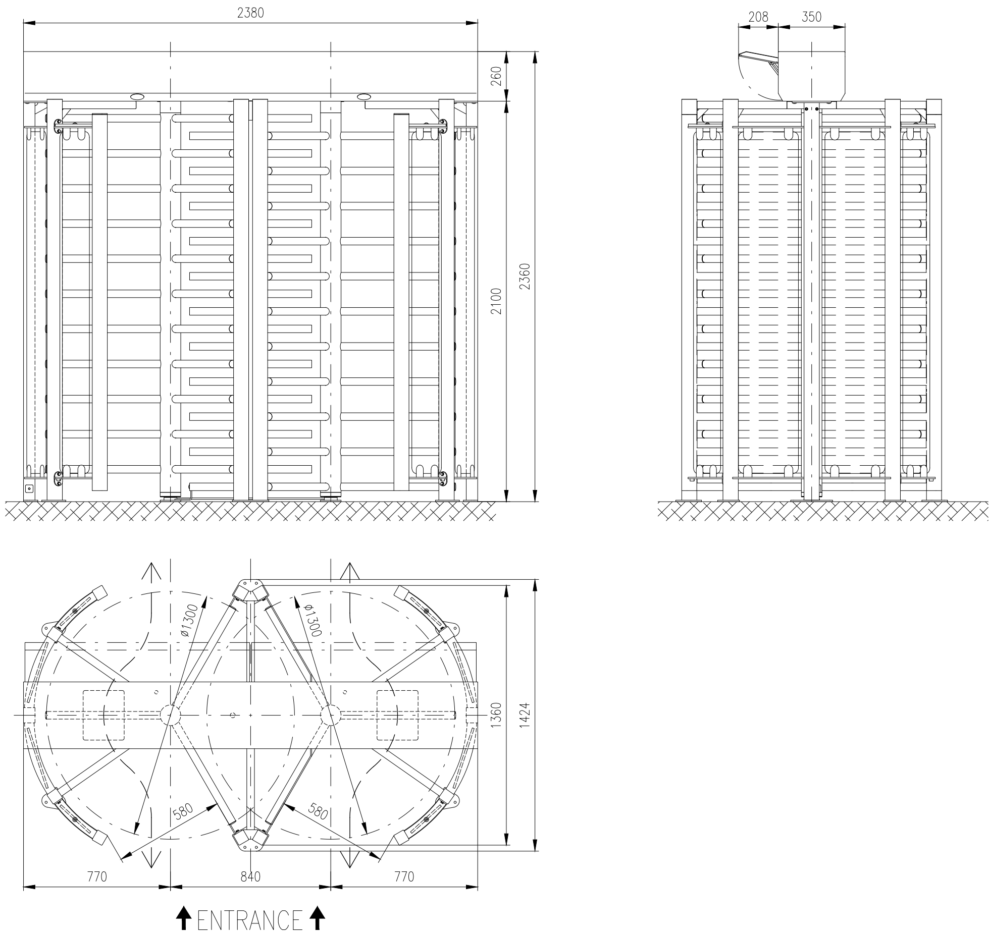
Motorized turnstile: REXON-ERA-4-DUO-GS
