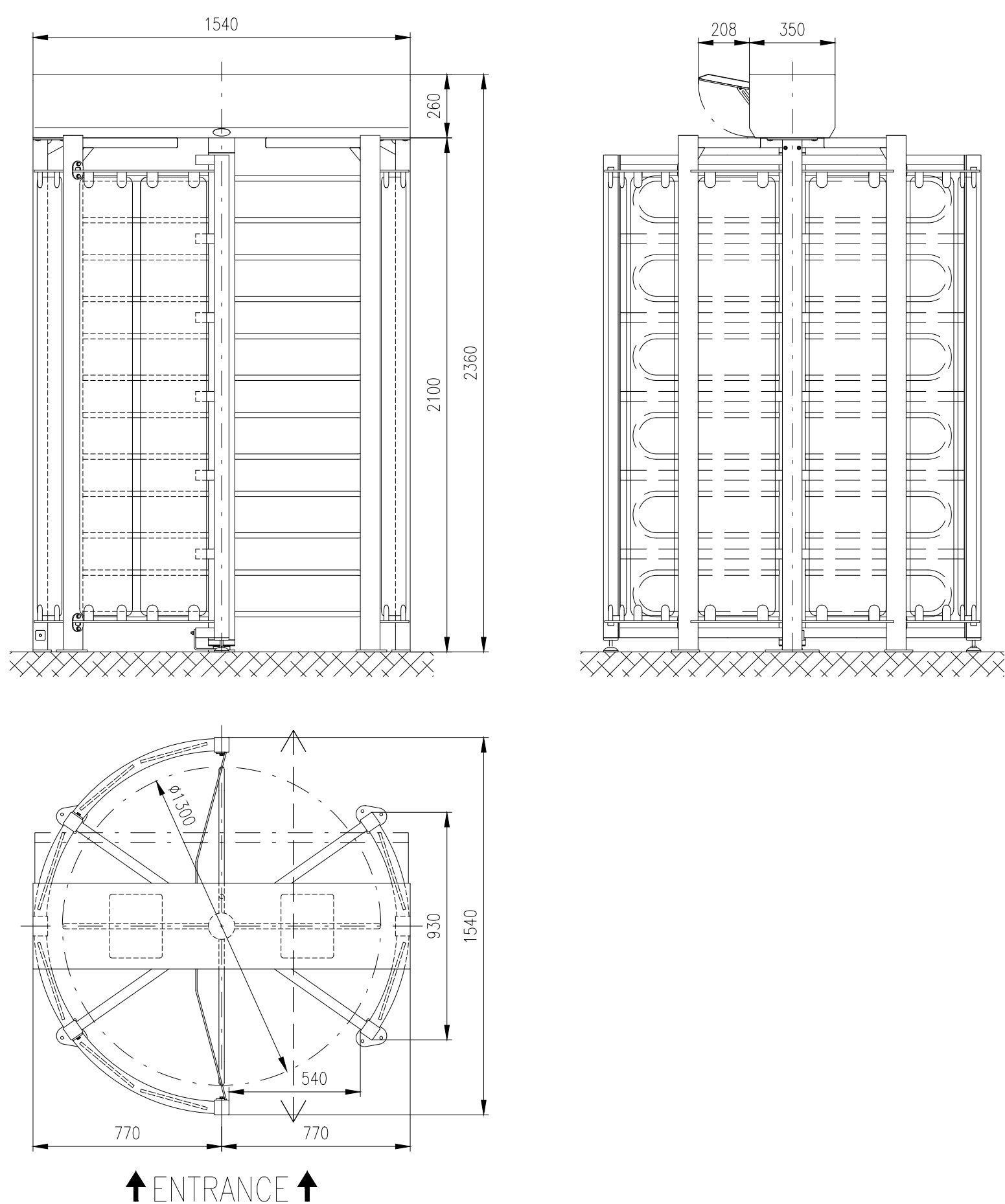
Motorized turnstile: REXON-ERA-4-FULL-GS-U
