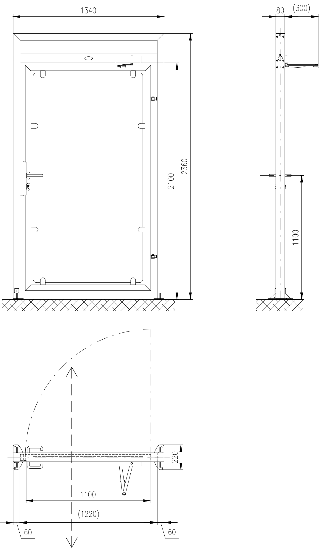
PedGate-GS: Left-Hand (manual lock)
