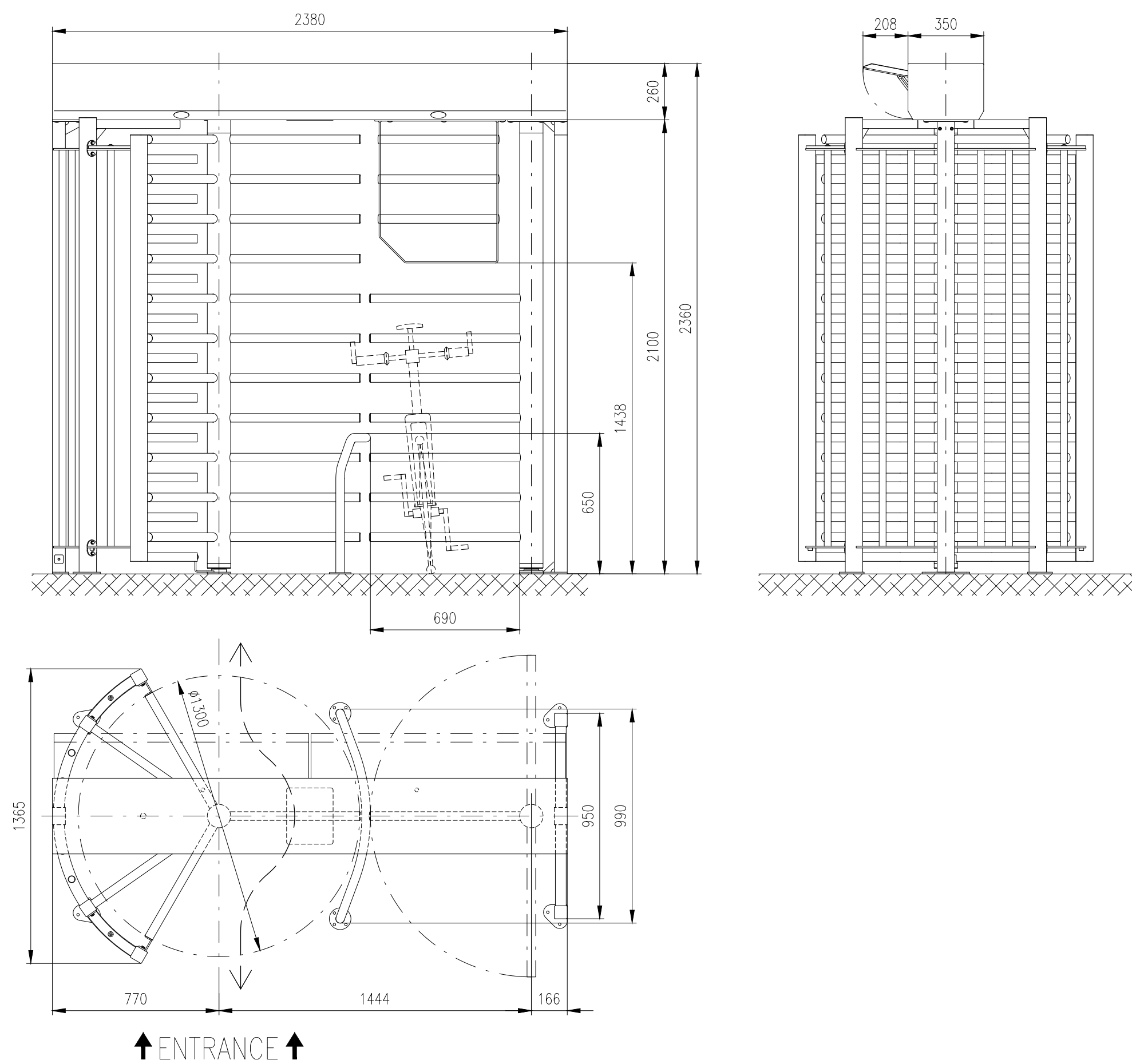
Motorized turnstile: REXON-ERA-3-BIKE
