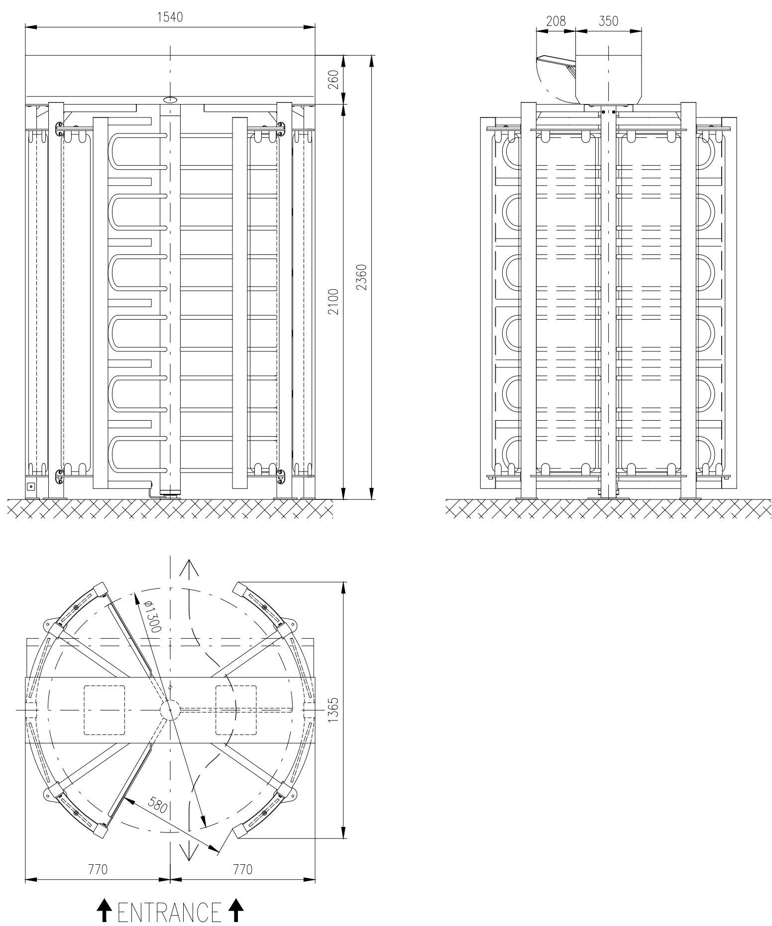
Motorized turnstile: REXON-ERA-3-FULL-GS-U
