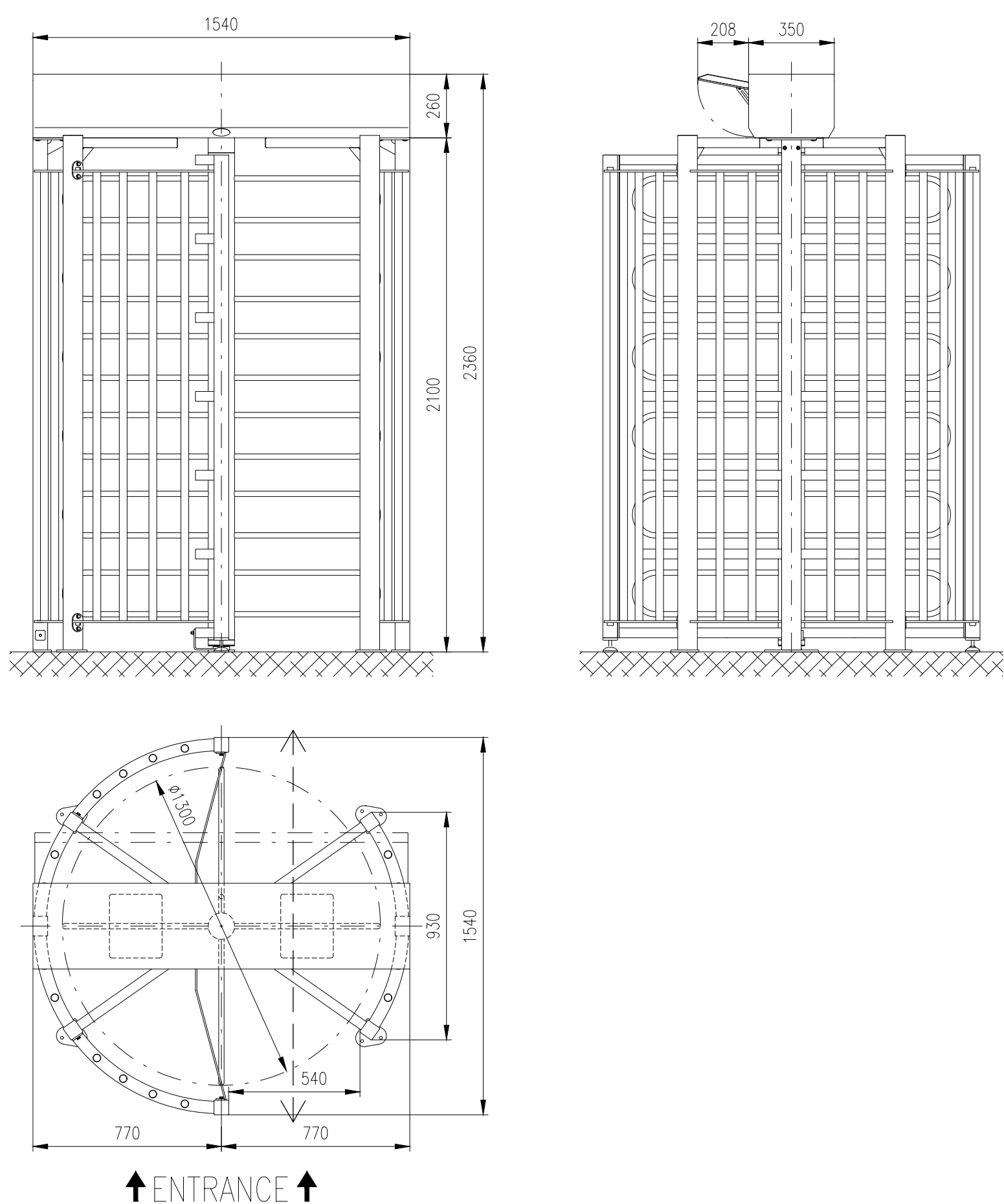
Motorized turnstile: REXON-ERA-4-FULL-U
