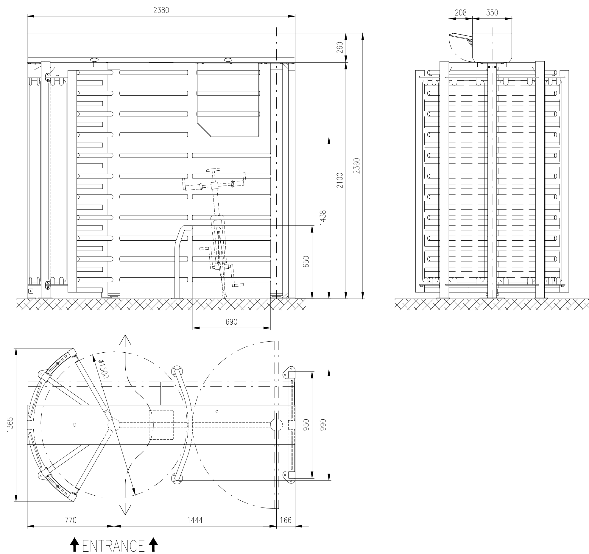
Motorized turnstile: REXON-ERA-3-BIKE-GS
