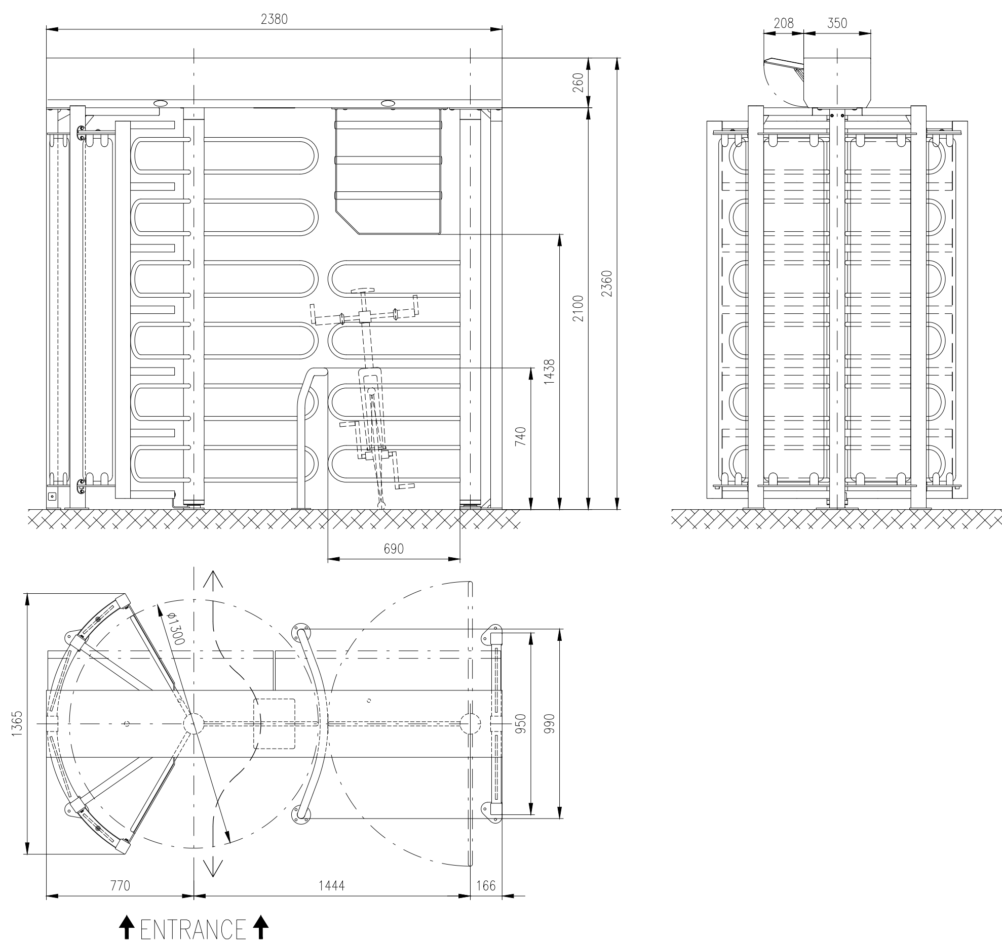
Motorized turnstile: REXON-ERA-3-BIKE-GS-U
