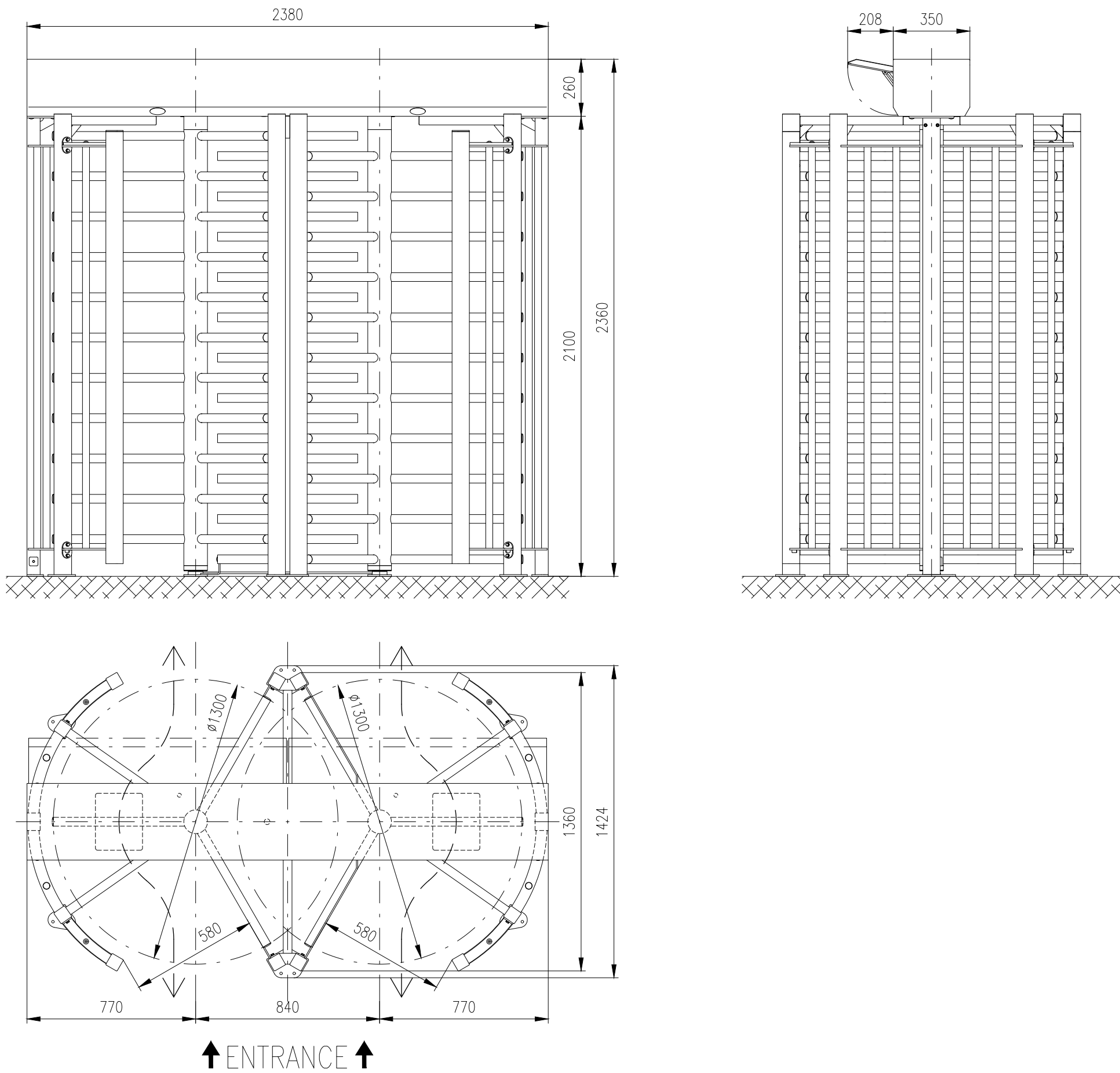
Motorized turnstile: REXON-ERA-4-DUO
