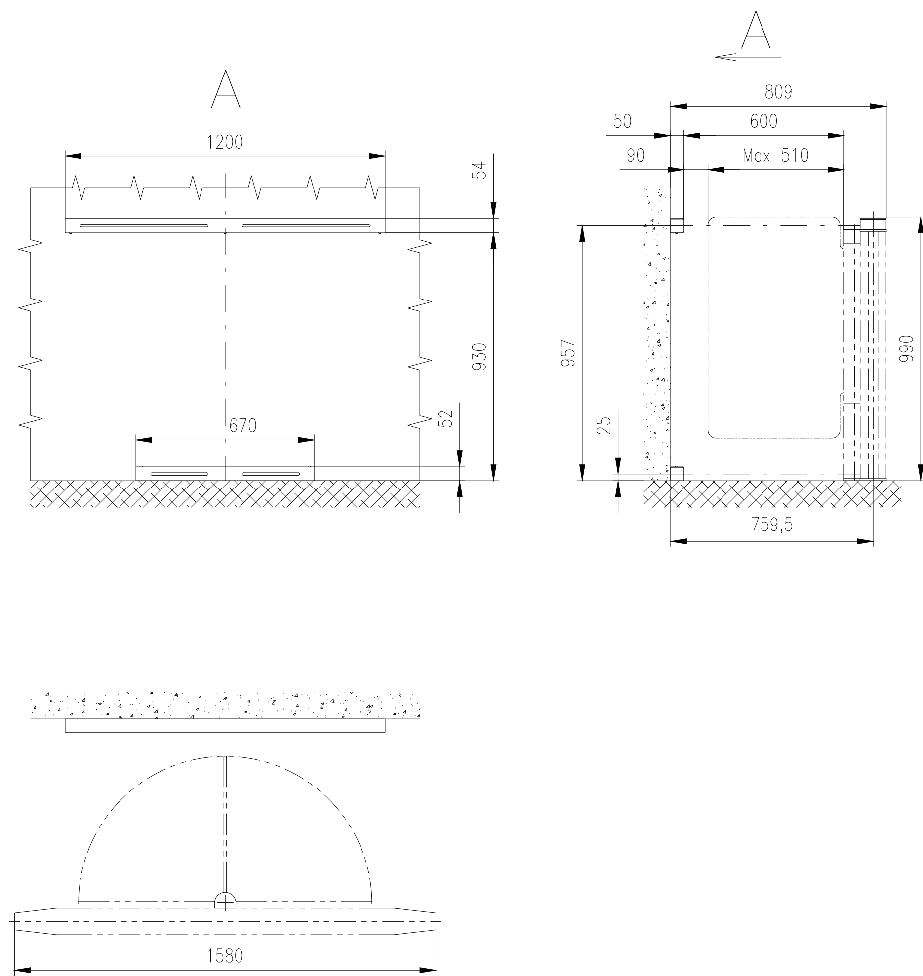
Modification for Sensors wall – Top mounted
