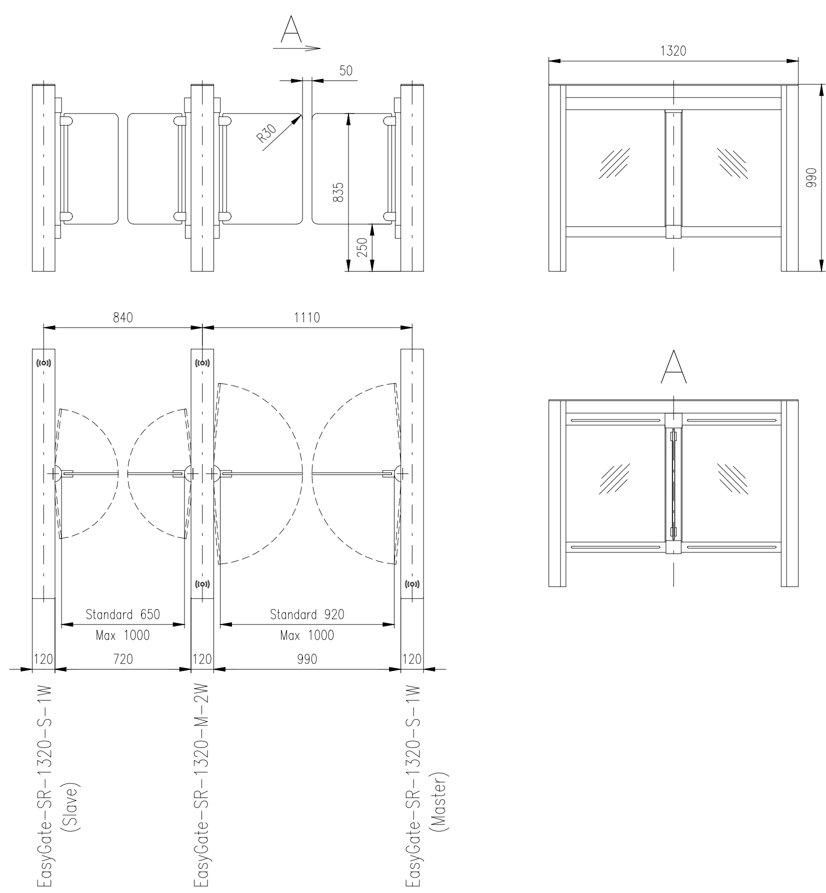
Turnstile: EasyGate-SR-1320 (Wing Light – Without Hinge Capping)
