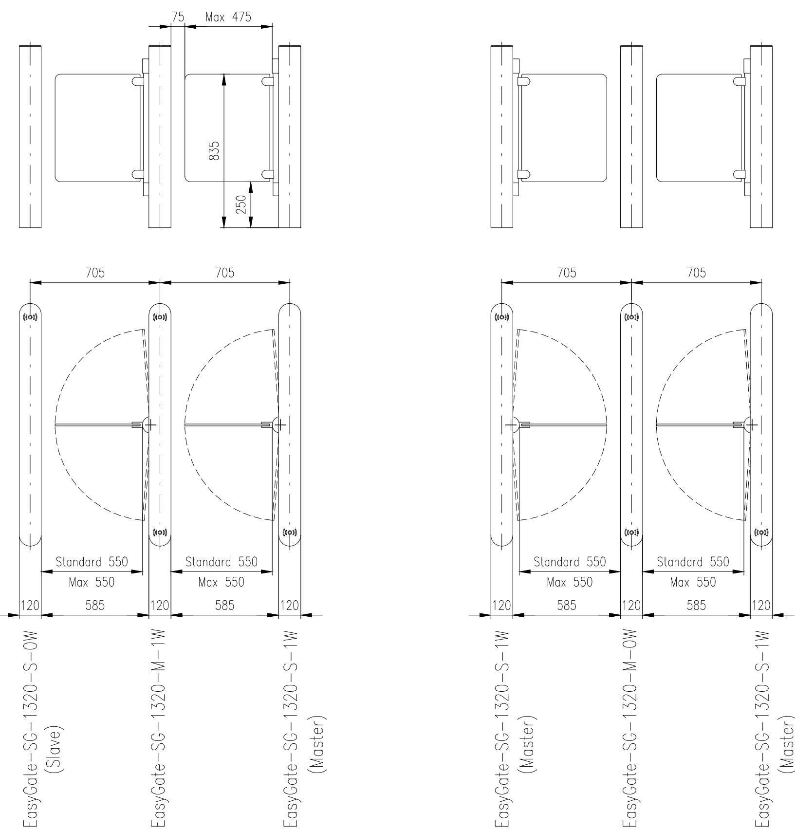
Turnstile: EasyGate-SG-1320 (Combination with single-wing variant)
