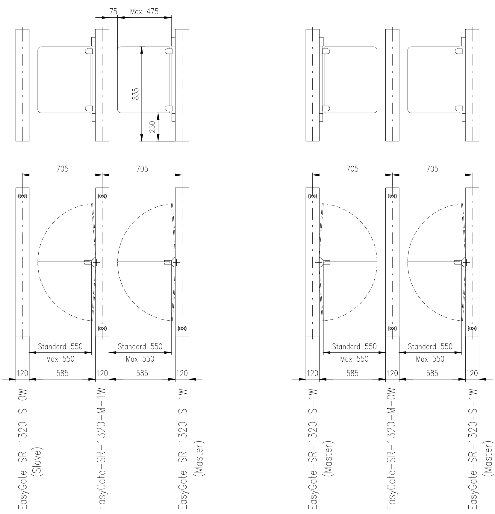
Turnstile: EasyGate-SR-1320 (Combination with single-wing variant)
