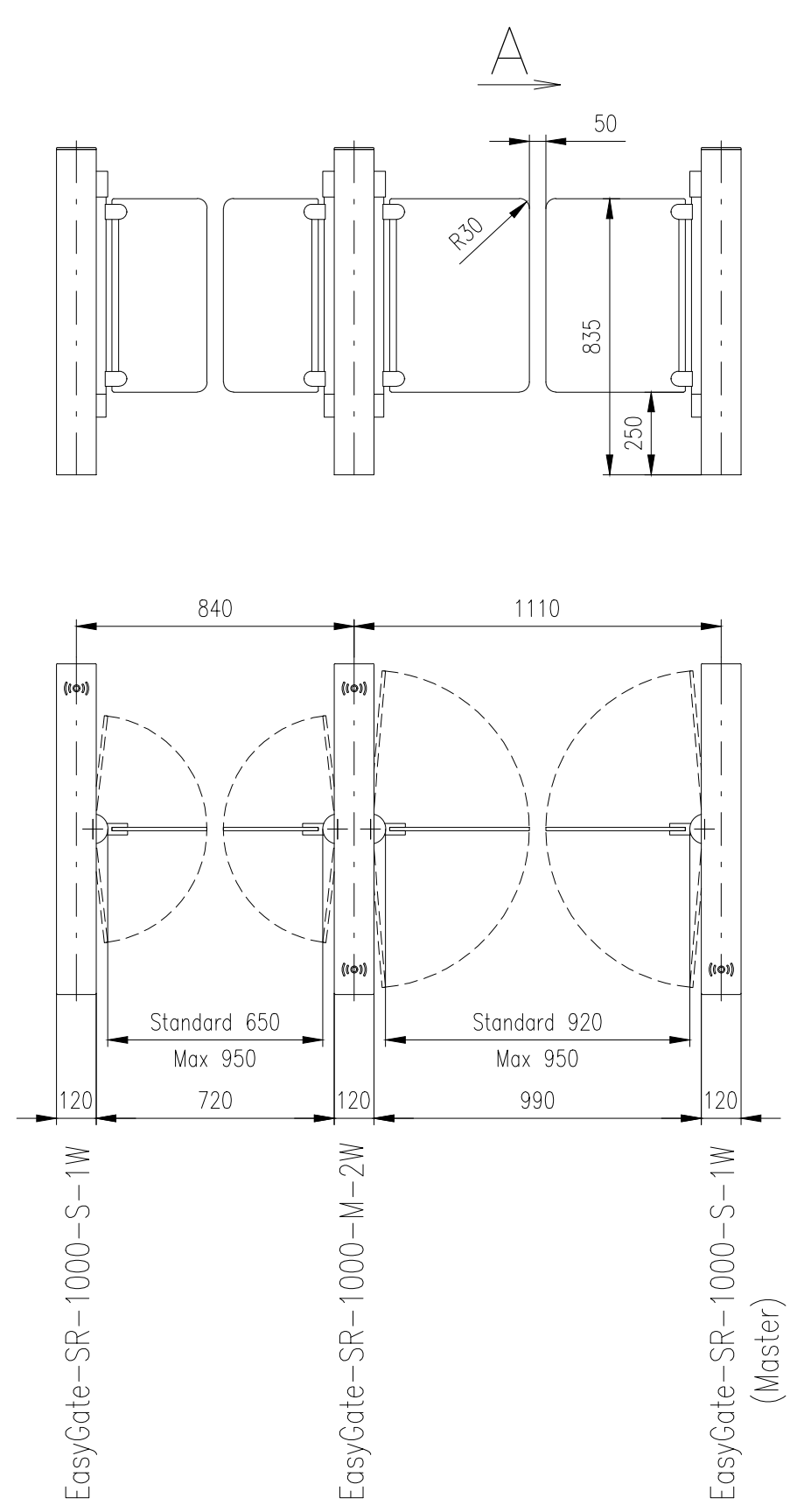
Turnstile: EasyGate–SR–1000 (Wing Light – Without Hinge Capping)
