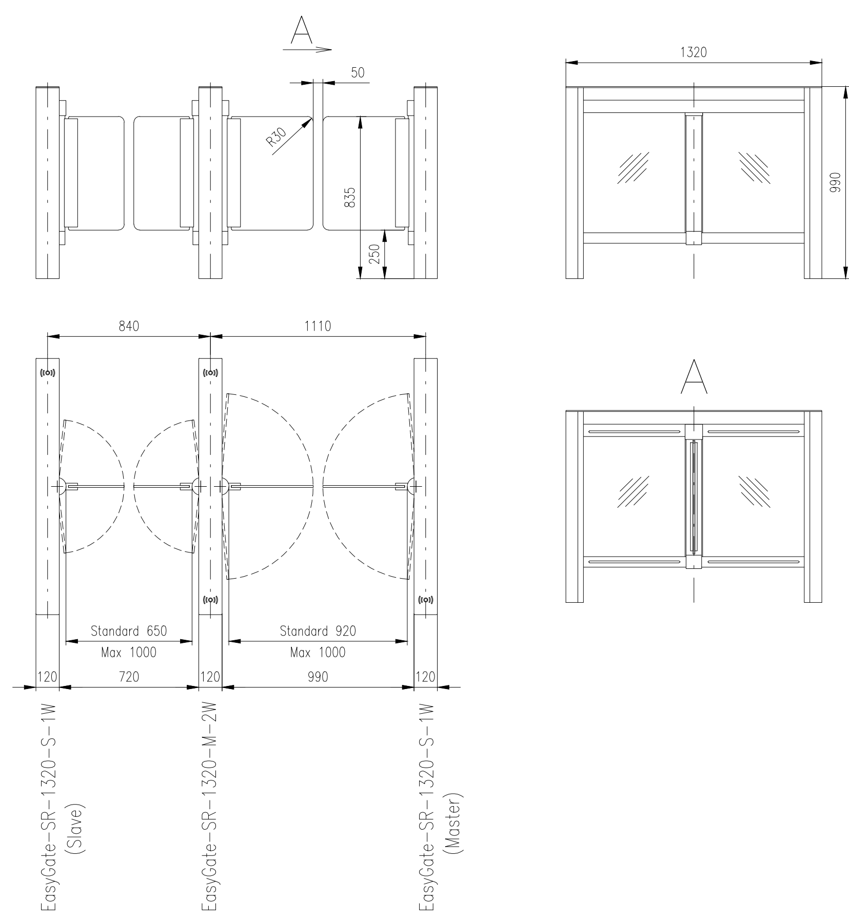
Turnstile: EasyGate-SR-1320 (Wing Light – Hinge Capping)
