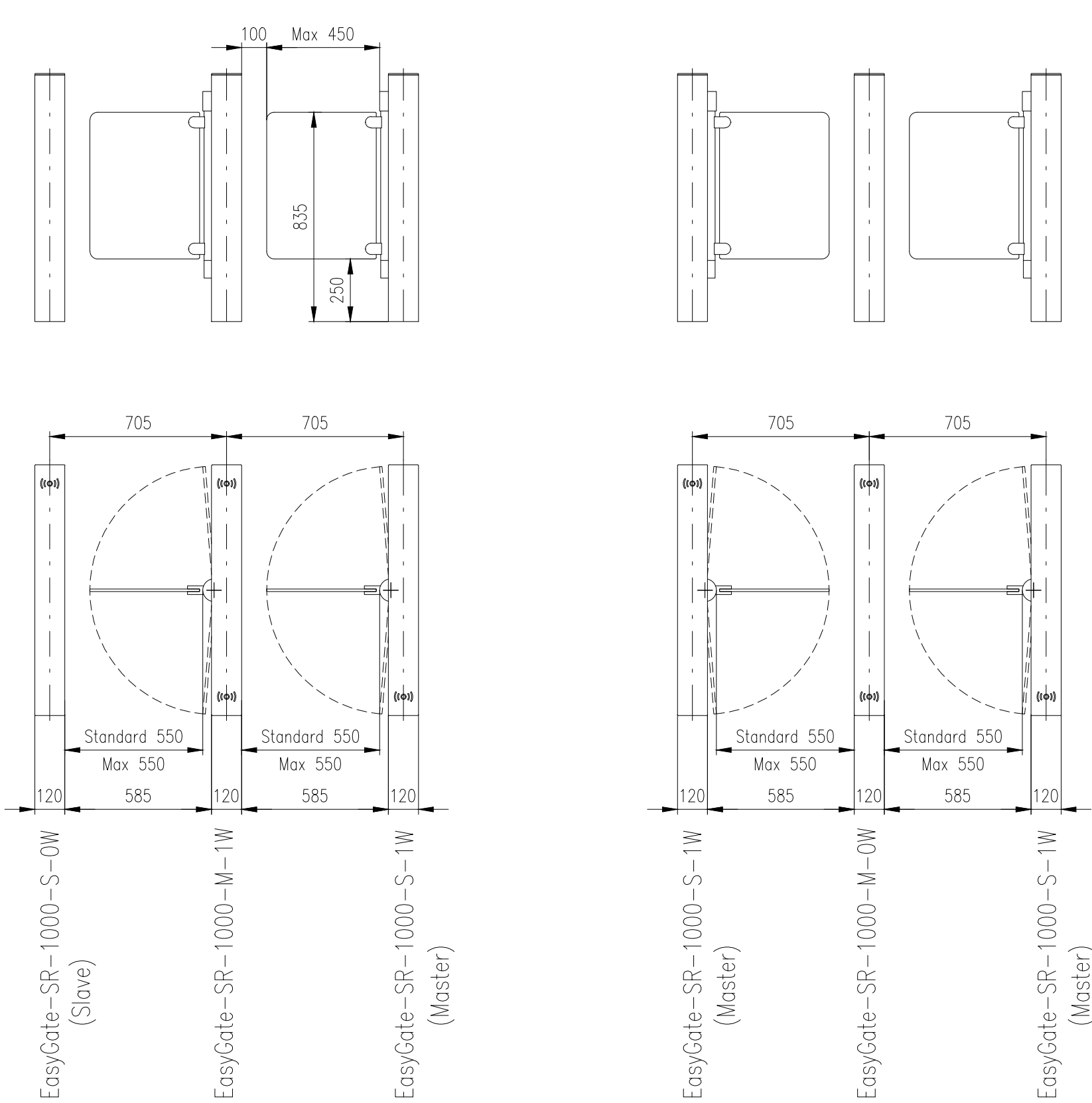
Turnstile: EasyGate–SR–1000 (Combination with single-wing variant)
