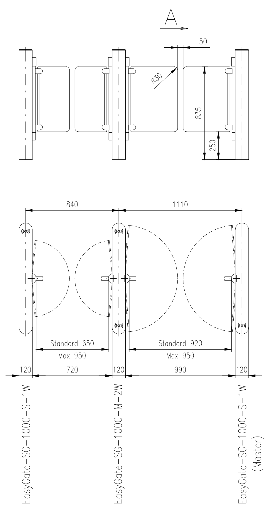
Turnstile: EasyGate-SG-1000 (Wing Light – Without Hinge Capping)
