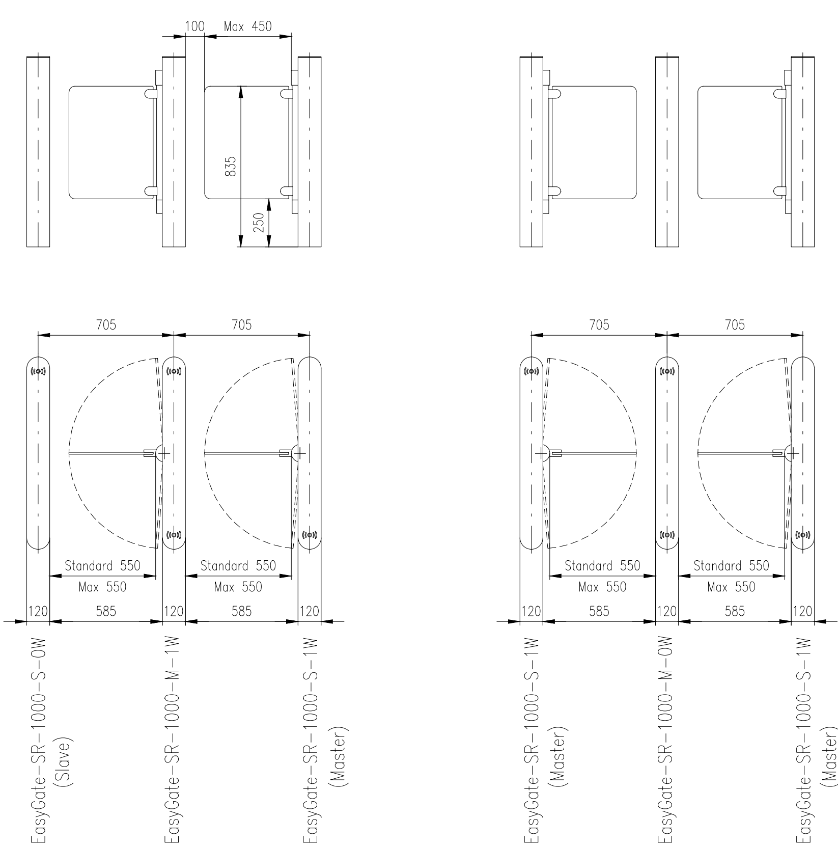
Turnstile: EasyGate-SG-1000 (Combination with single-wing variant)
