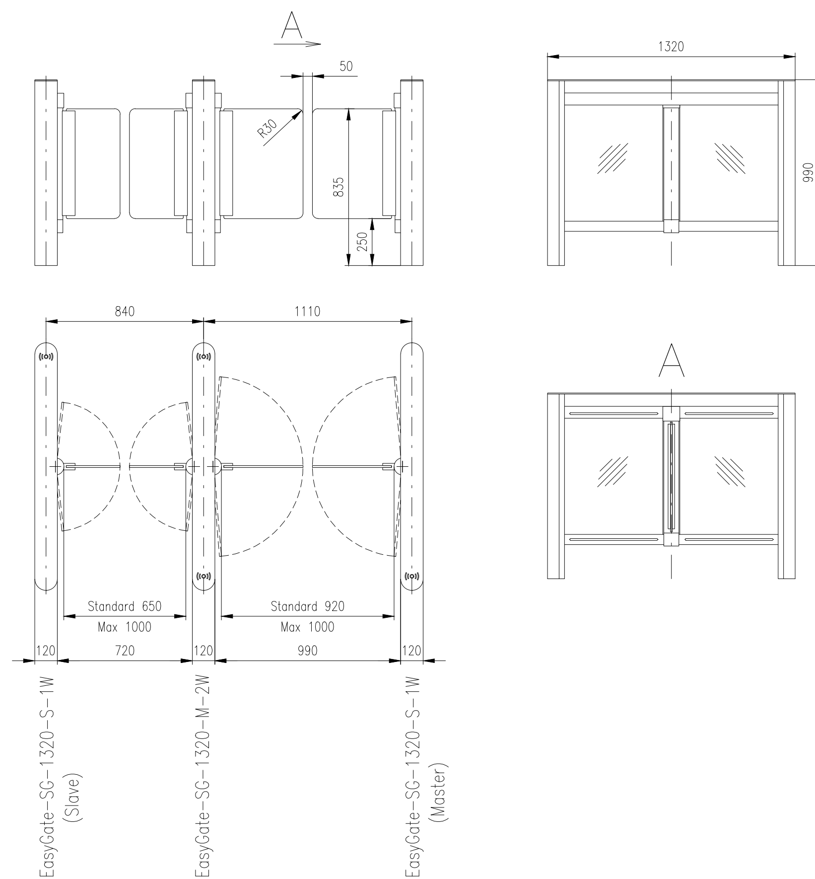
Turnstile: EasyGate-SG-1320 (Wing Light – Hinge Capping)
