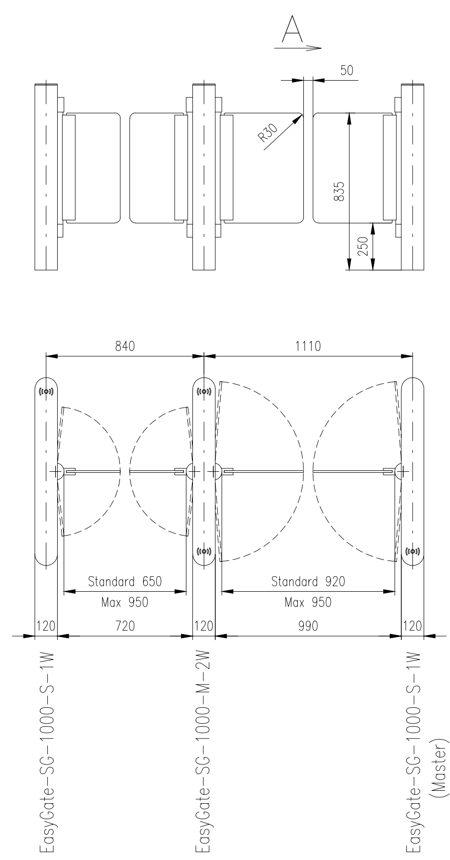
Turnstile: EasyGate-SG-1000 (Wing Light – Hinge Capping)
