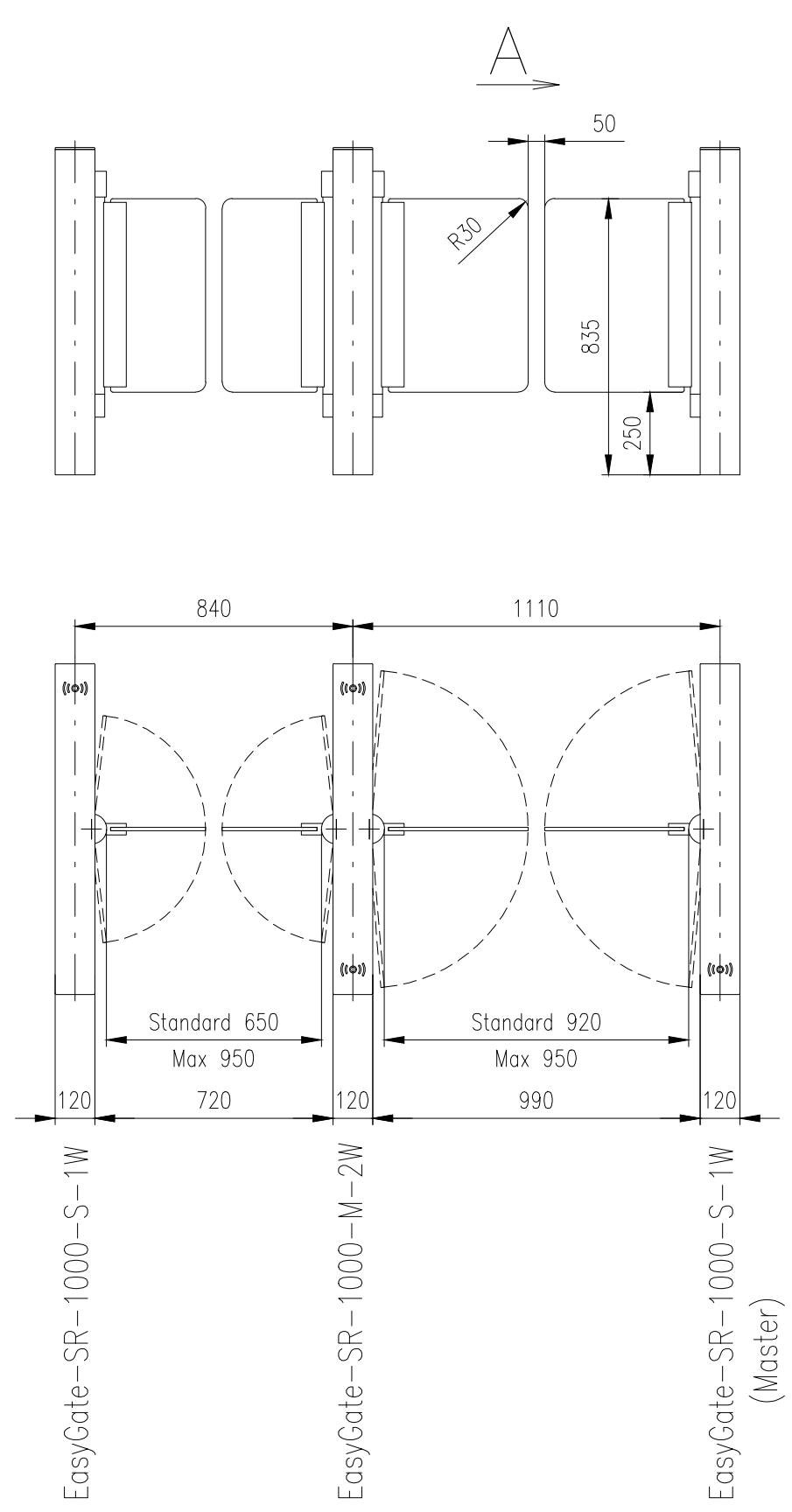
Turnstile: EasyGate–SR–1000 (Wing Light – Hinge Capping)
