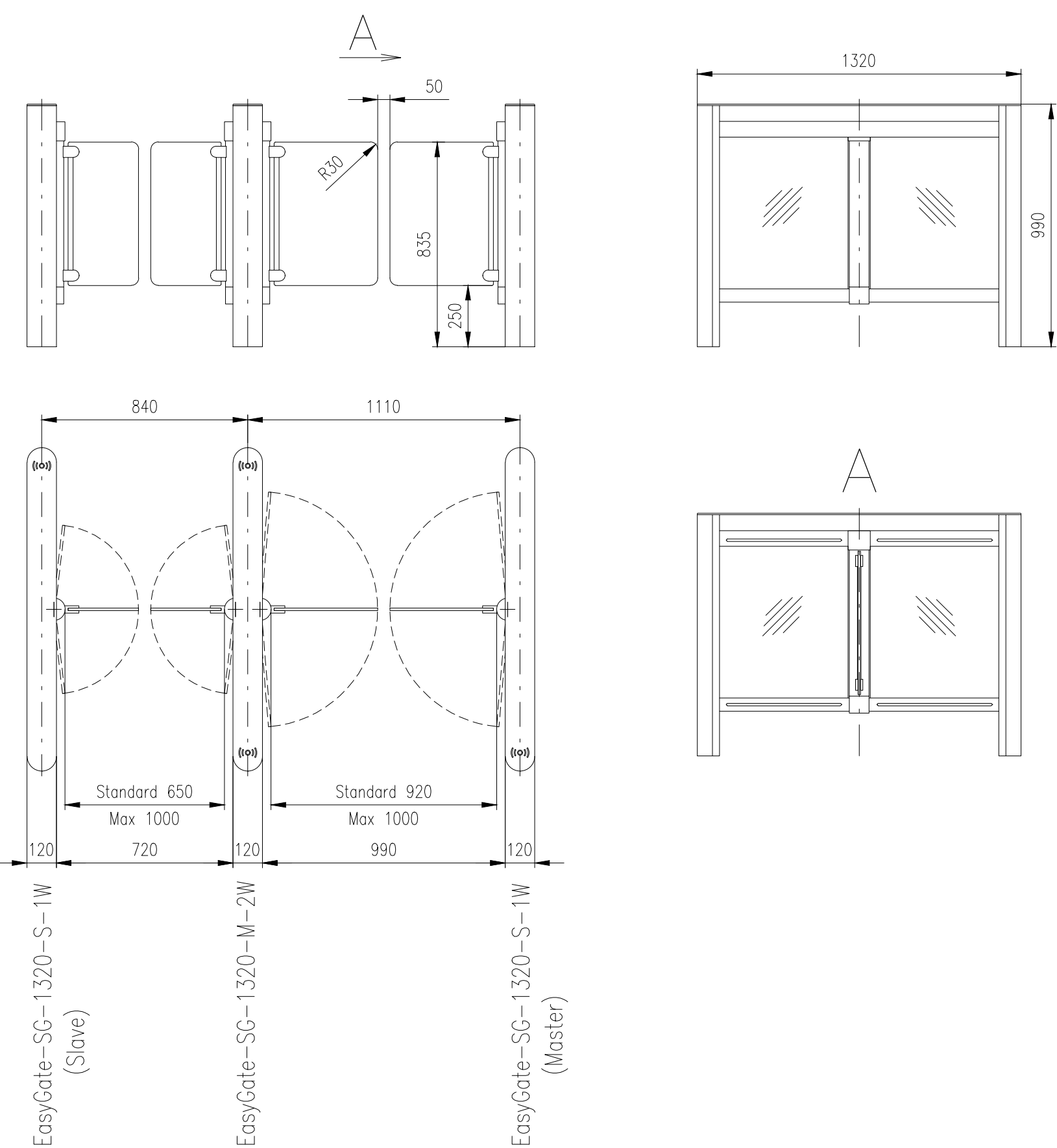
Turnstile: EasyGate-SG-1320 (Wing Light – Without Hinge Capping)
