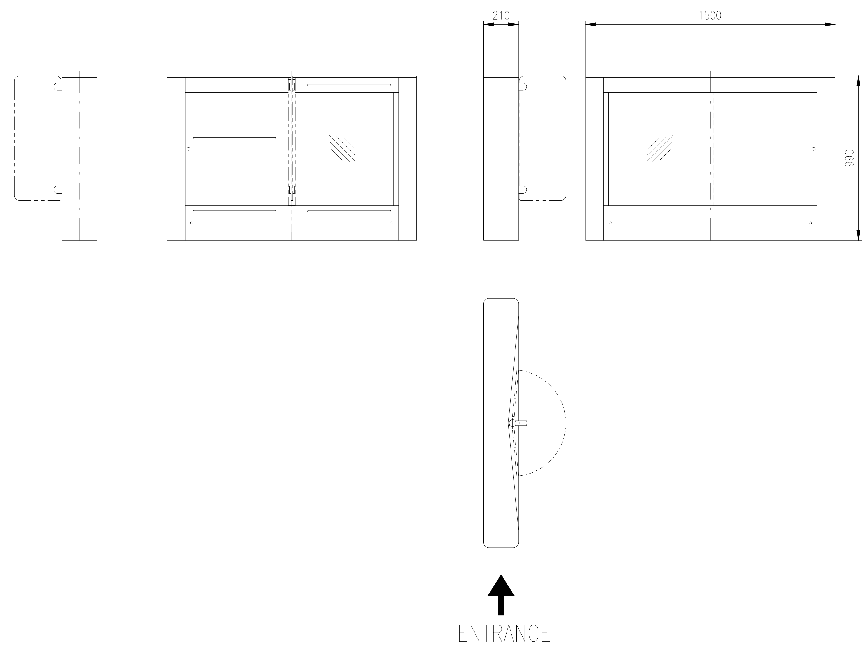
Turnstile: EasyGate–SBG–M–1W
