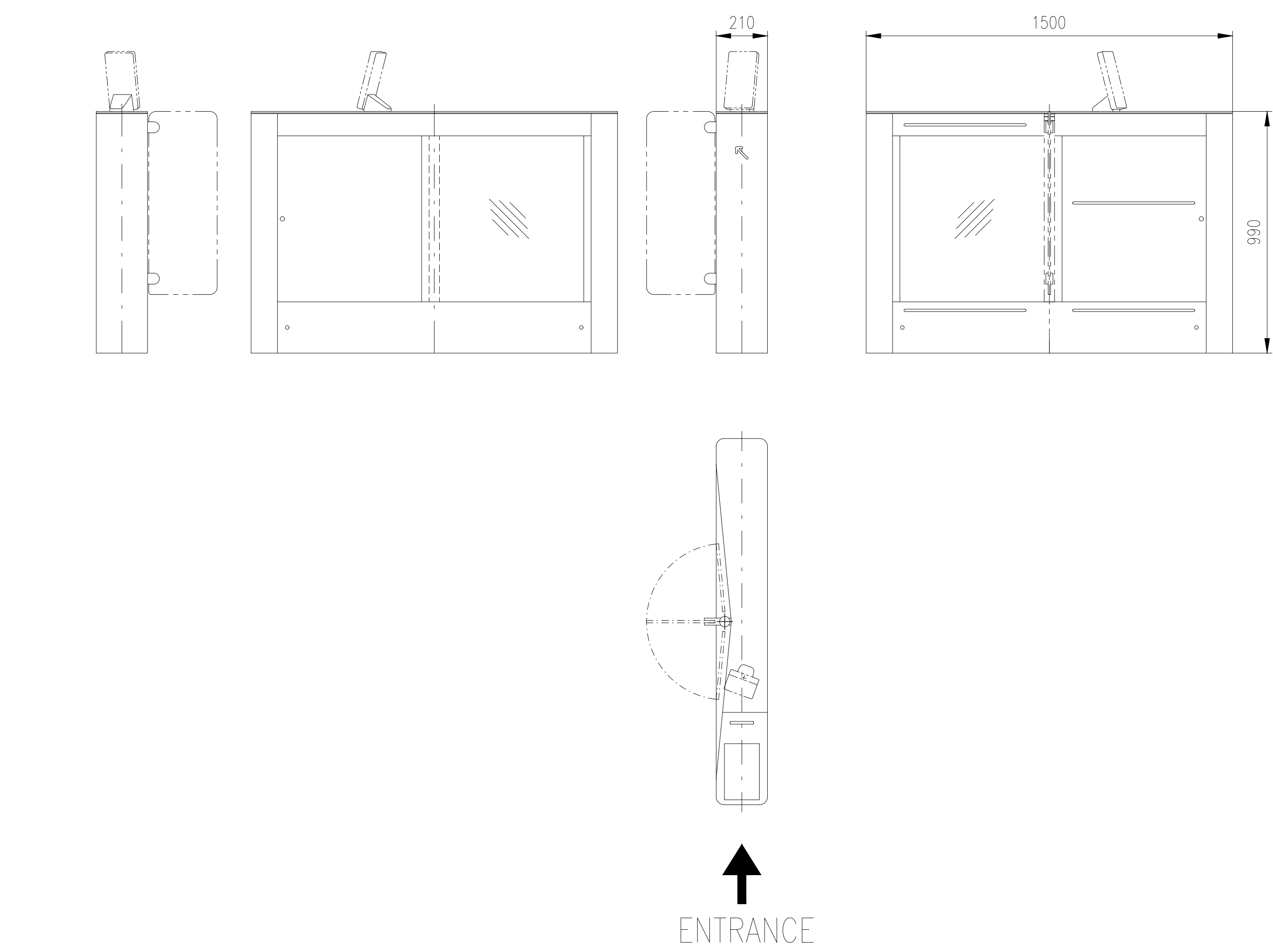
Turnstile: EasyGate–SBG–M–2W
