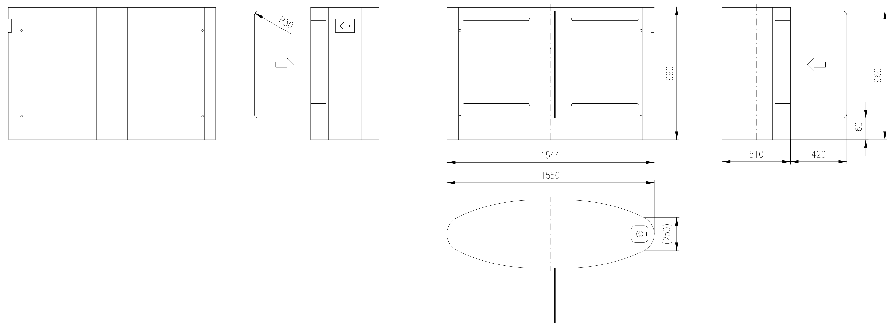
Turnstile: EASYGATE-LG-W-S (wide)
