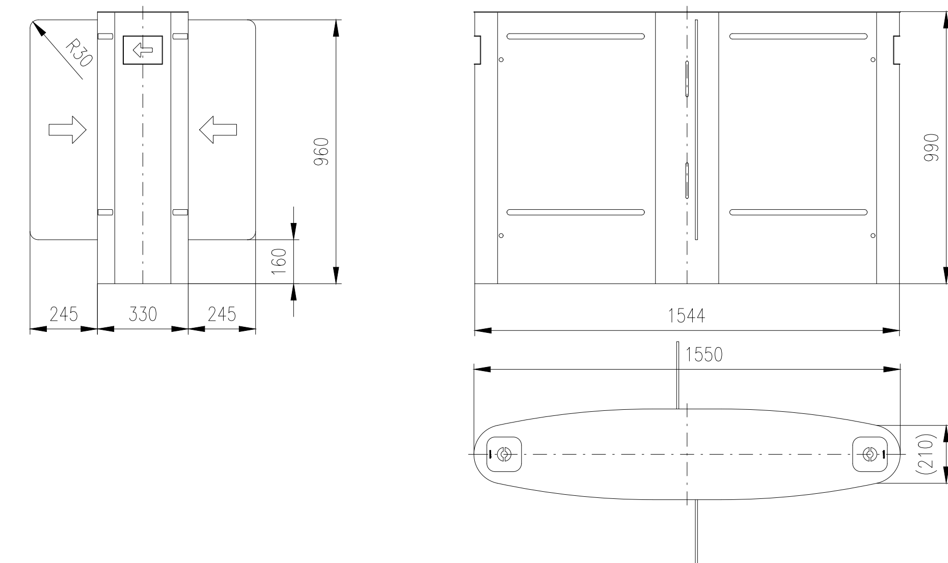
Turnstile: EASYGATE-LG-W-M (wide/narrow)
