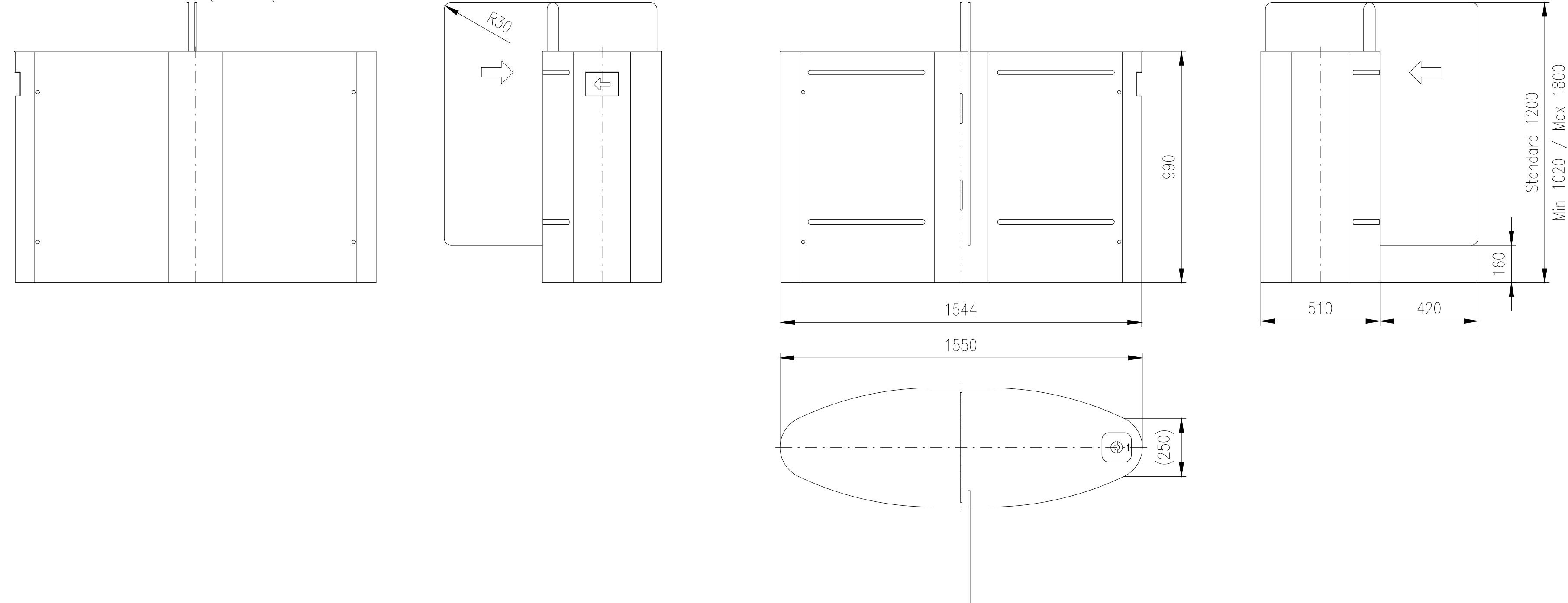
Turnstile: EASYGATE-LG-N-S (narrow)
