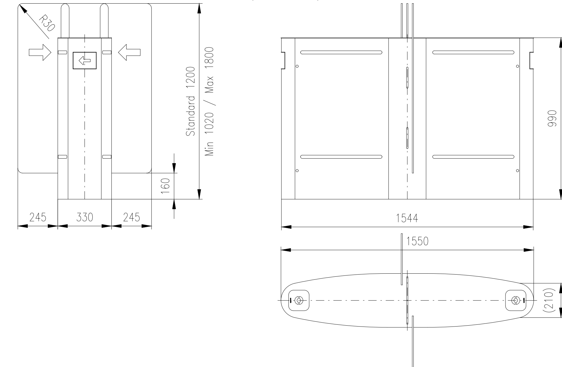
Turnstile: EASYGATE-LG-W-M (wide/narrow)
