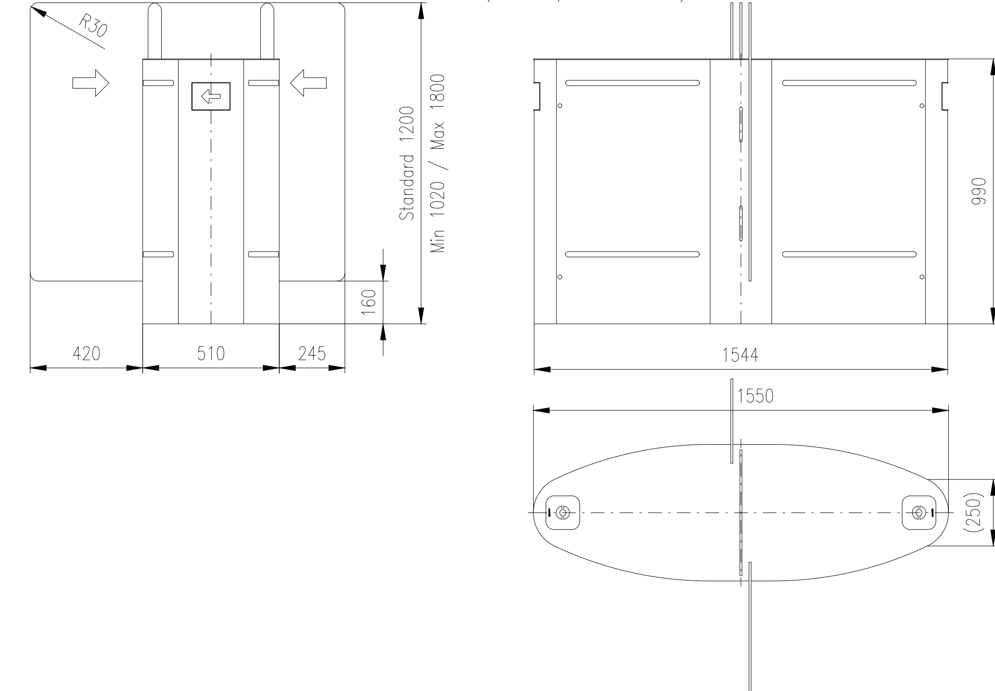
Turnstile: EASYGATE-LG-N-M (narrow)
