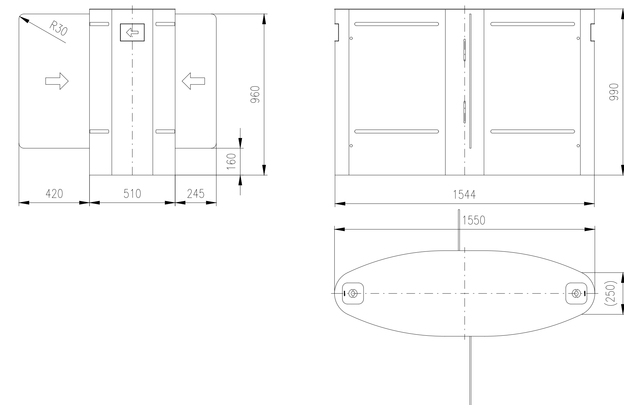
Turnstile: EASYGATE-LG-W-M (wide/narrow)
