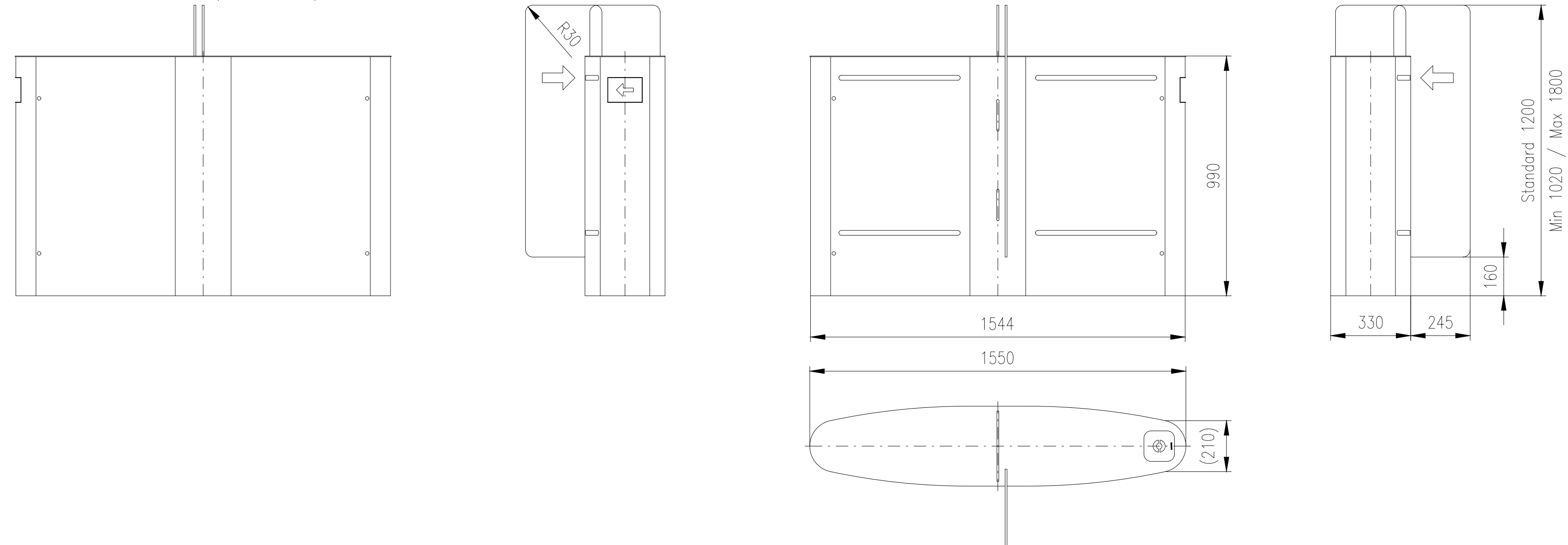
Turnstile: EASYGATE-LG-W-S (wide)
