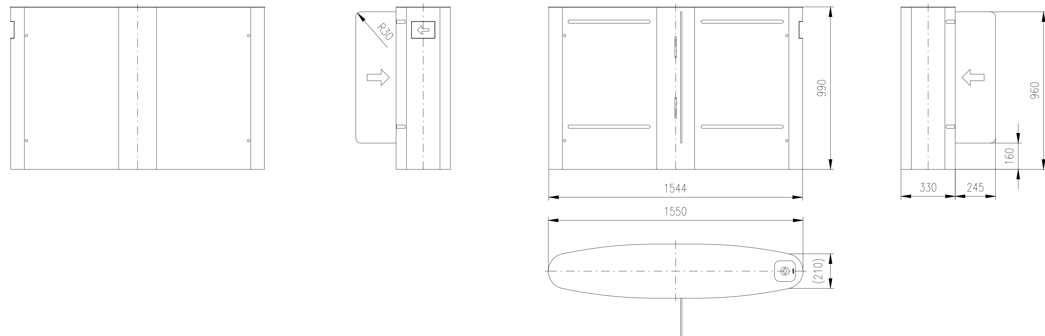
Turnstile: EASYGATE-LG-W-S (wide)
