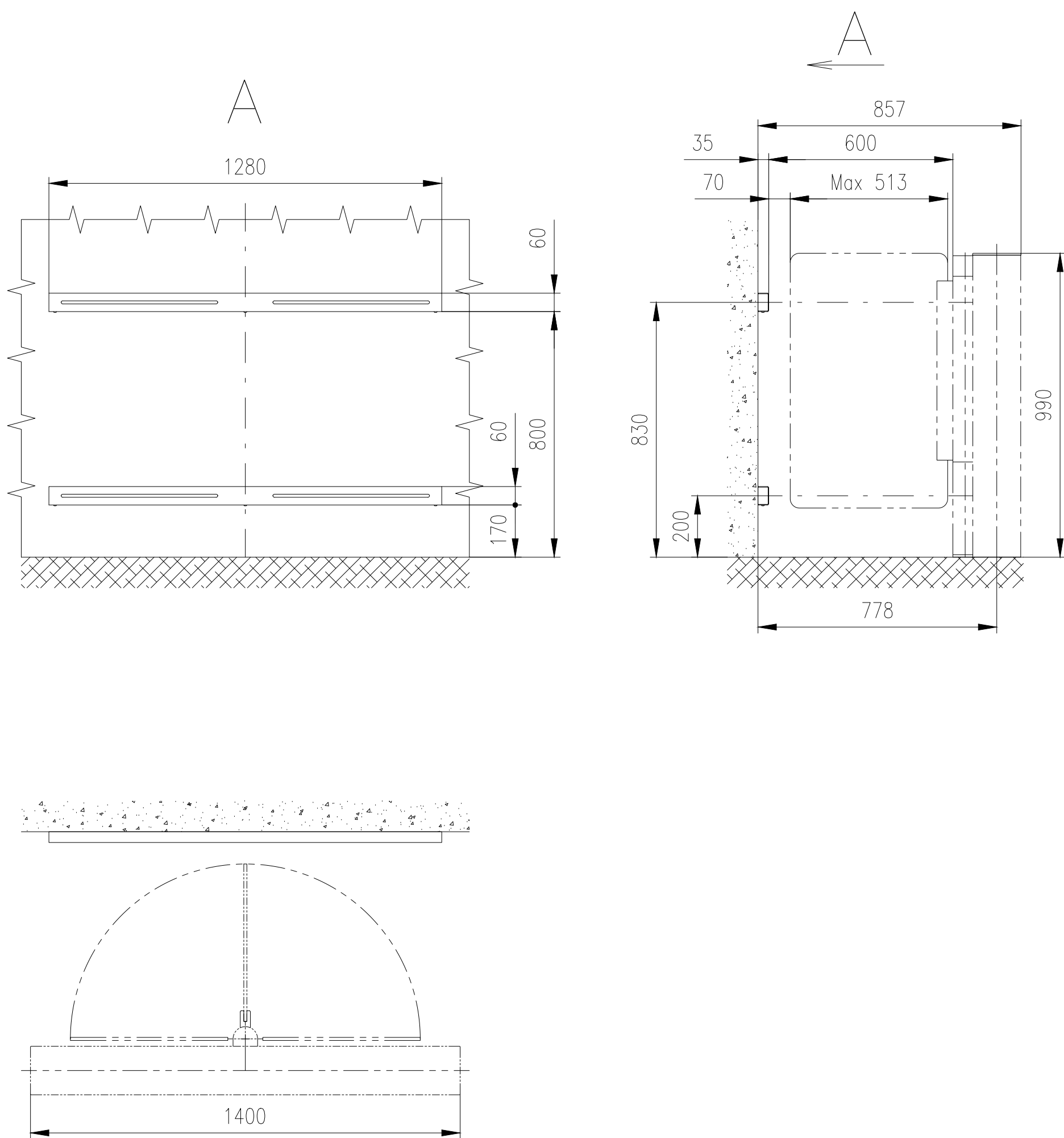
Modification for Sensors wall – Top mounted
