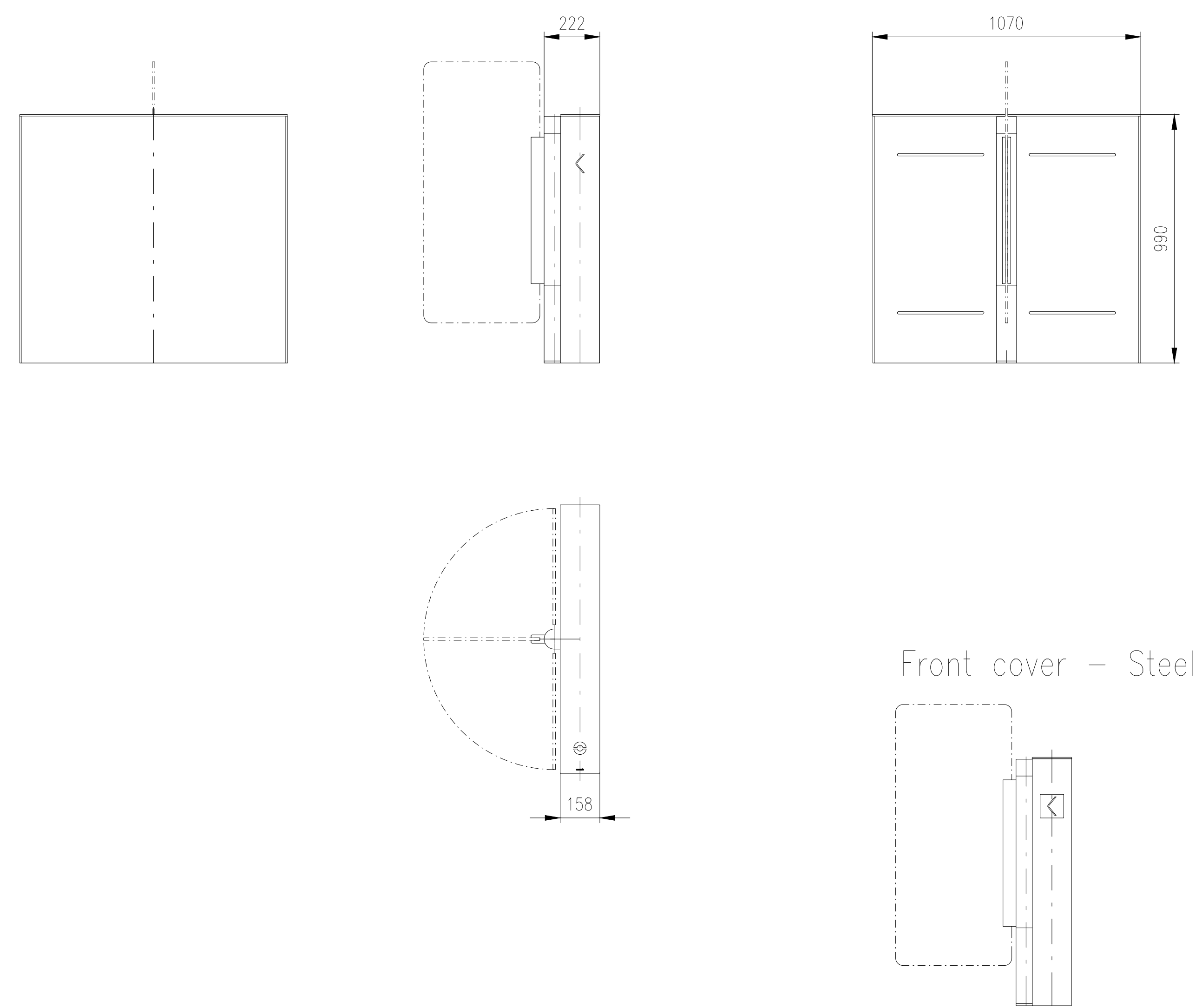
Modification for Sensors wall – Flush mounted
