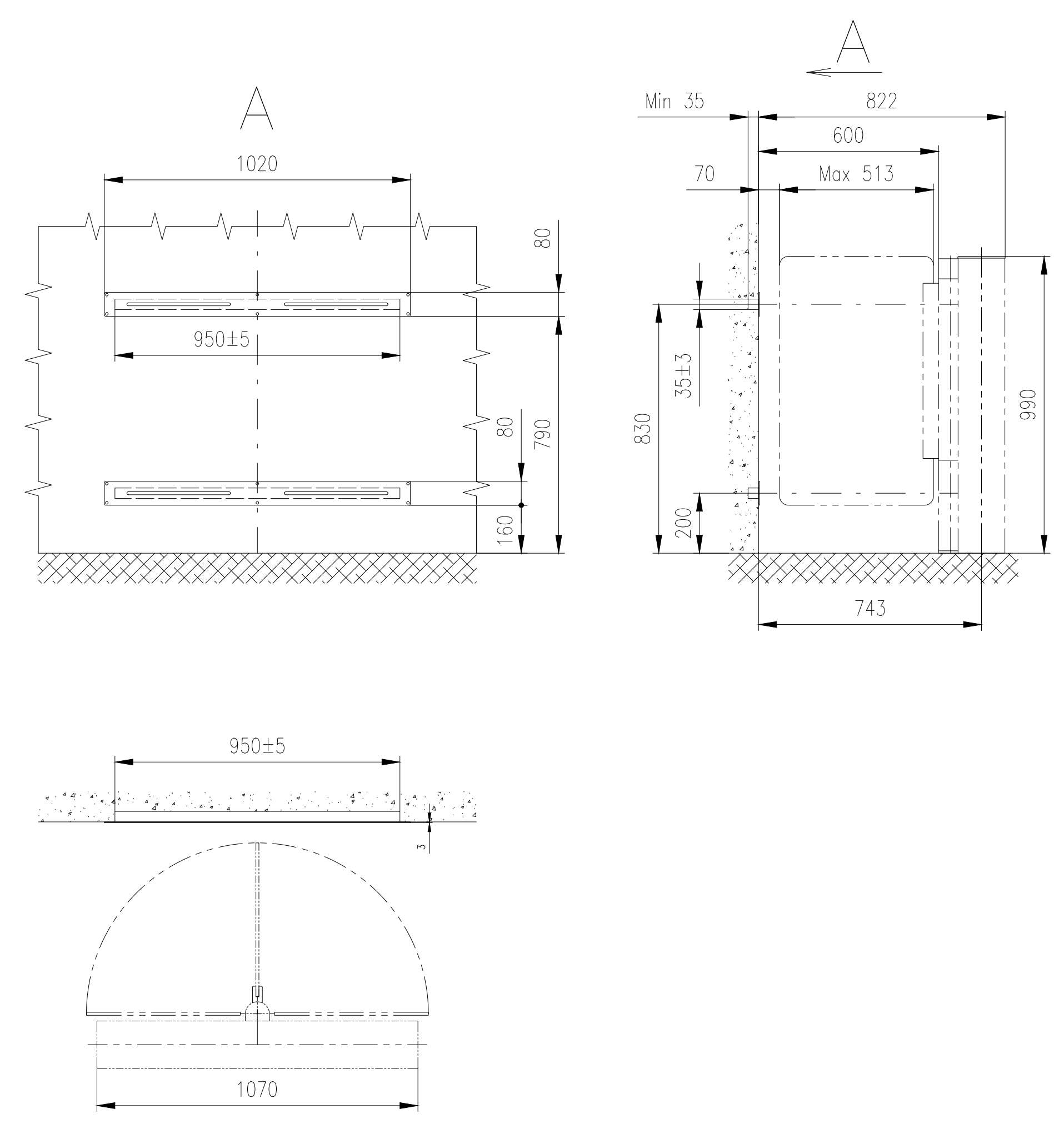
Modification for Sensors wall – Flush mounted
