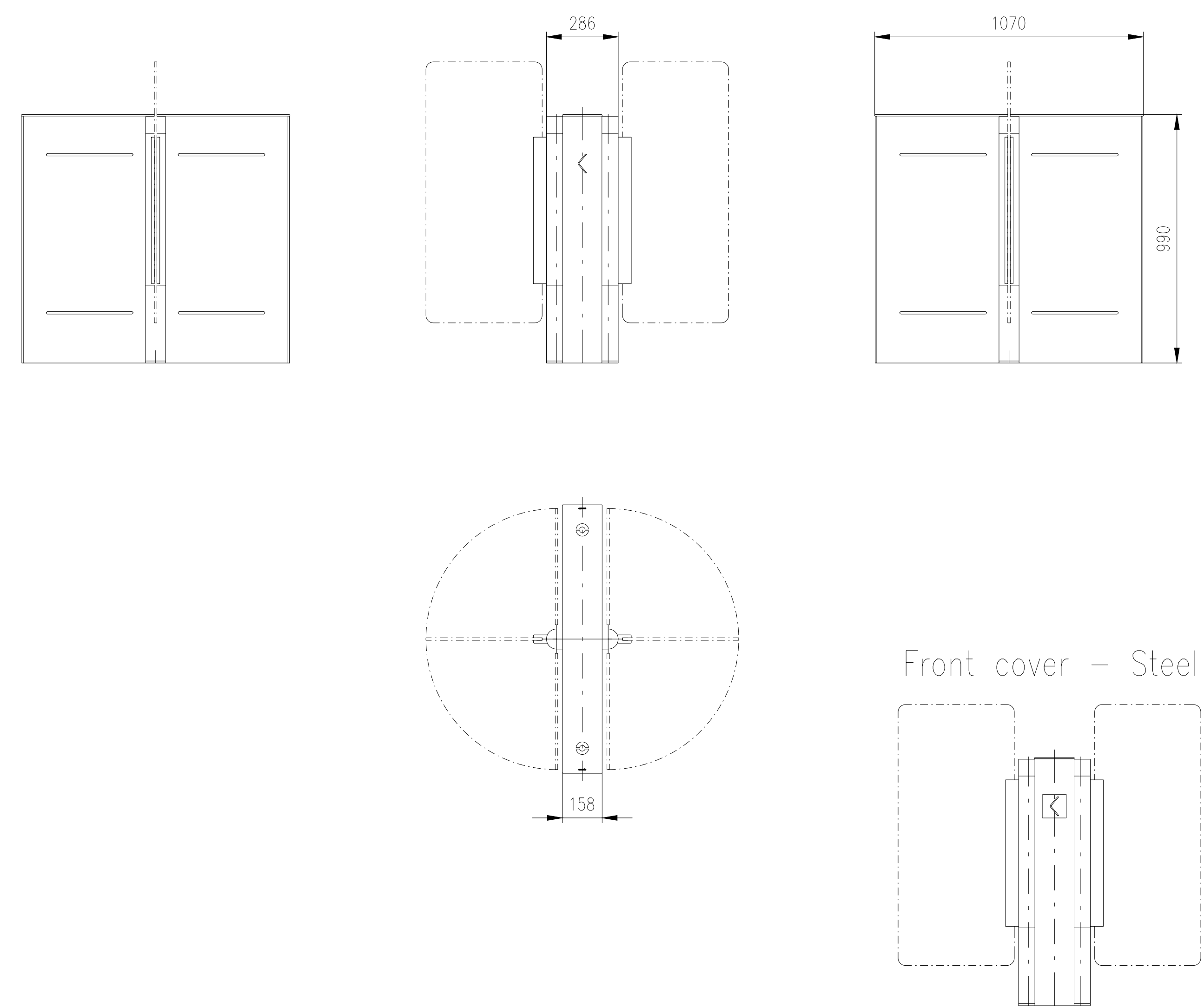
Turnstile: EasyGate–LC–S–0W–Short
