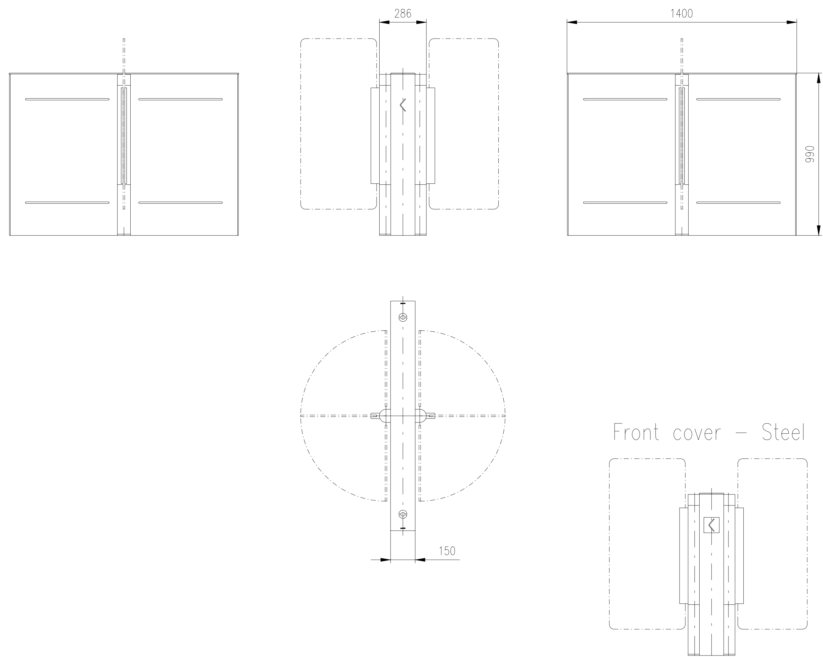
Turnstile: EasyGate–LC–S–0W
