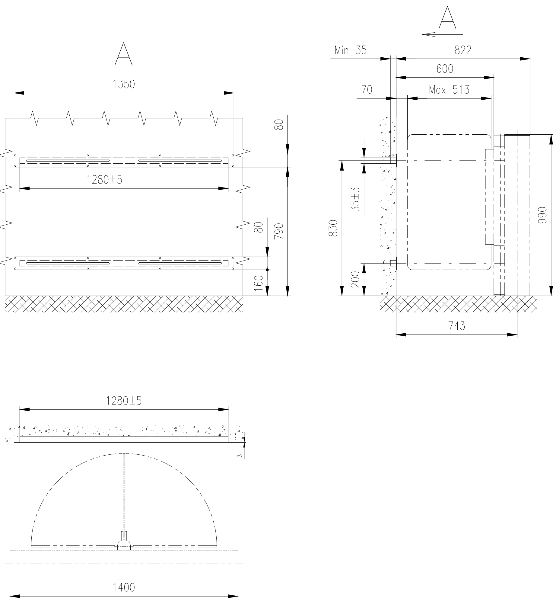
Modification for Sensors wall – Flush mounted
