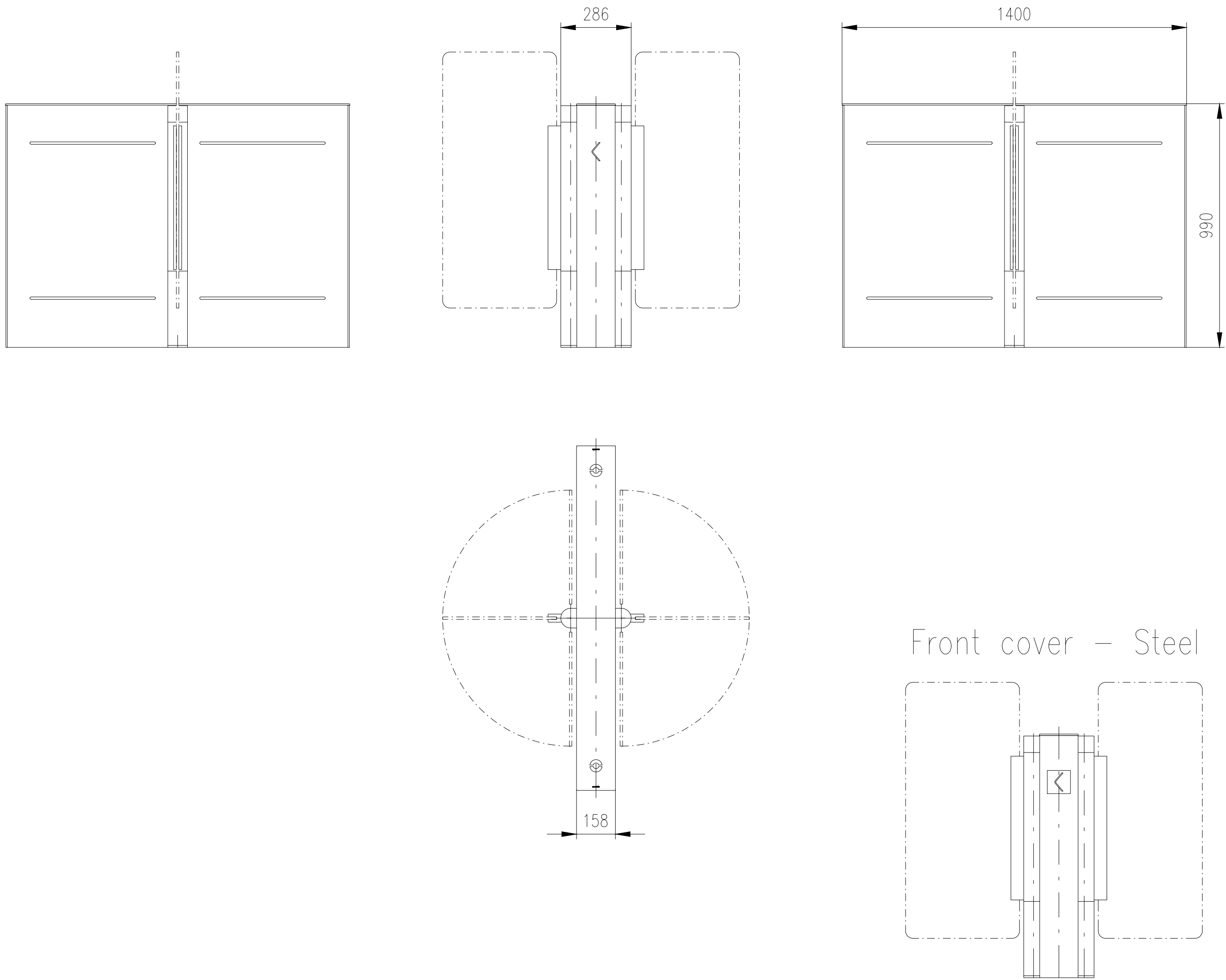
Turnstile: EasyGate–LC–S–0W
