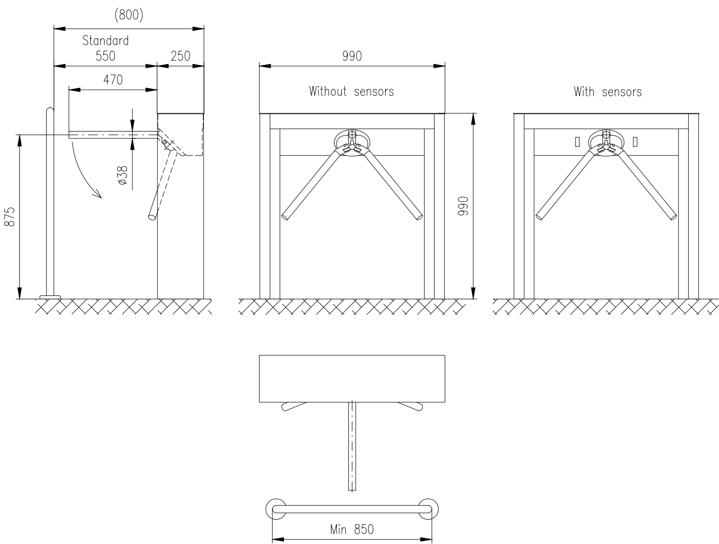
Turnstile: BAR–One–R–DropArm
