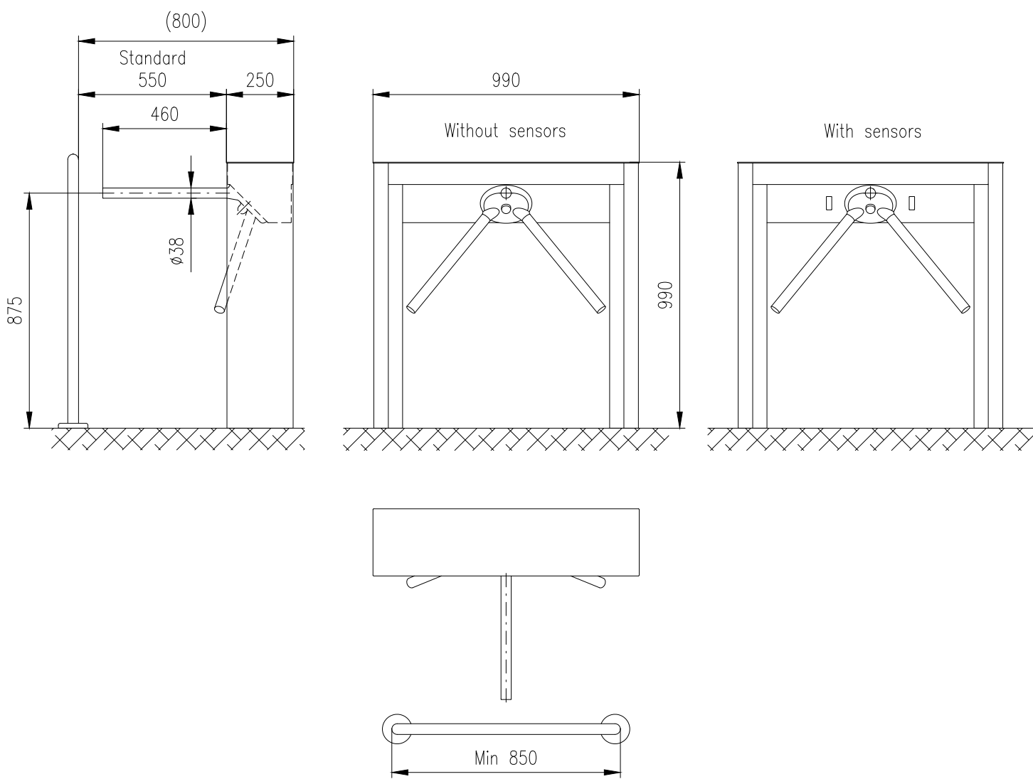
Turnstile: BAR–One–R–Tripod
