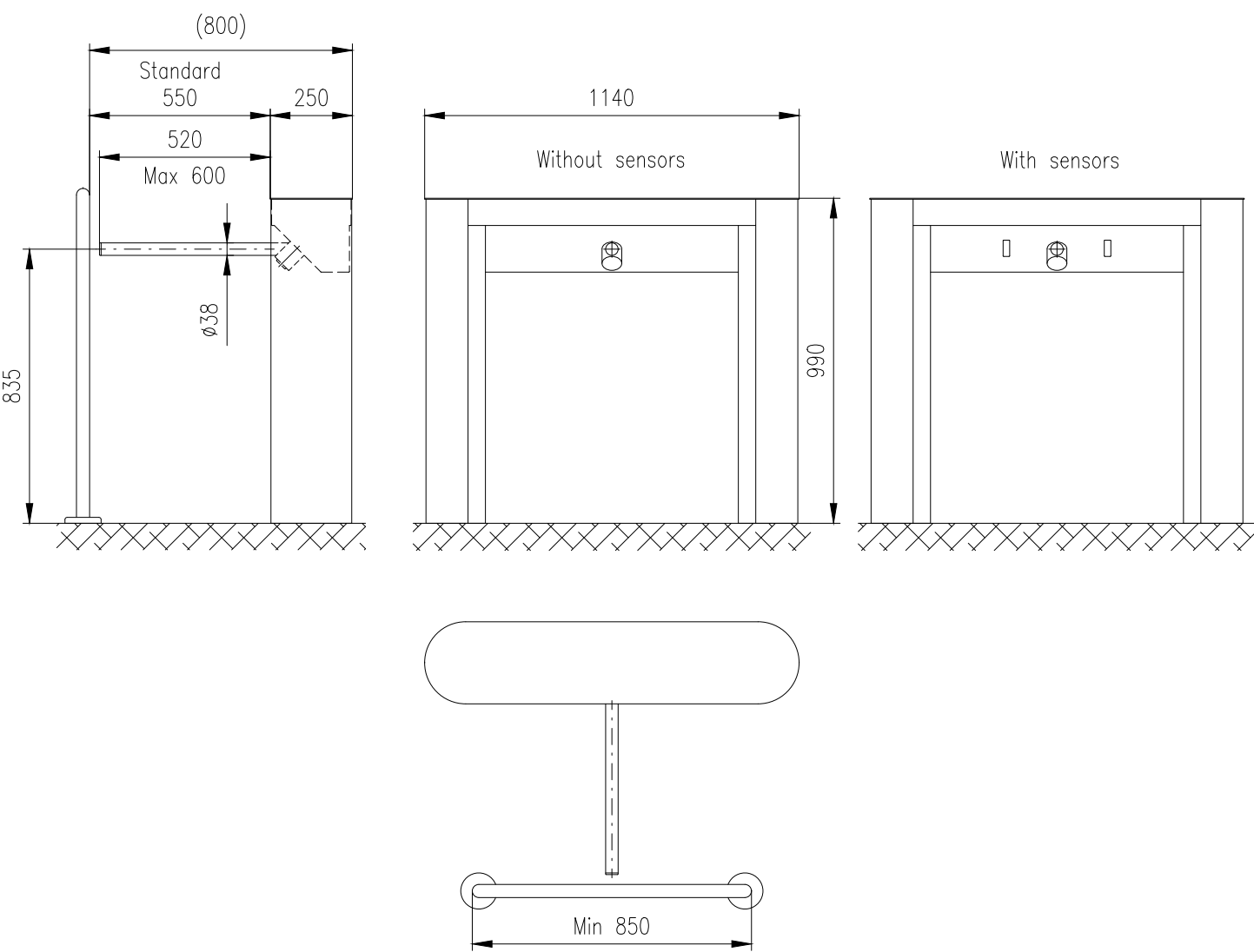
Turnstile: BAR–One–G–Unipod
