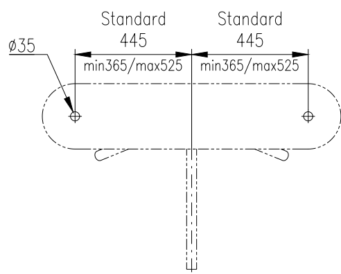
Terminal post hole – Variant 2
