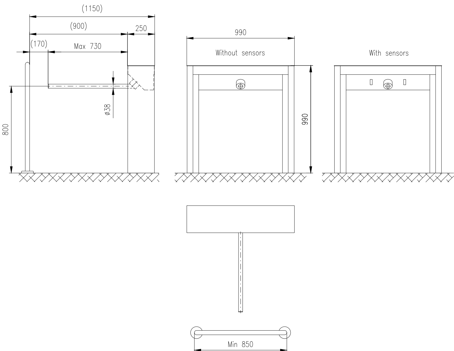
Turnstile: BAR–One–R–Gate
