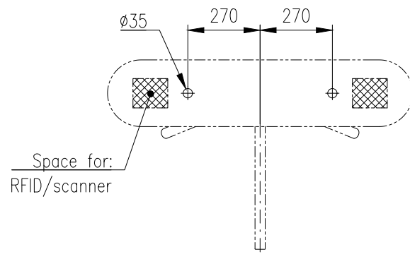
Easy Scan – Glass window
