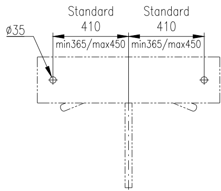
Terminal post hole – Variant 2
