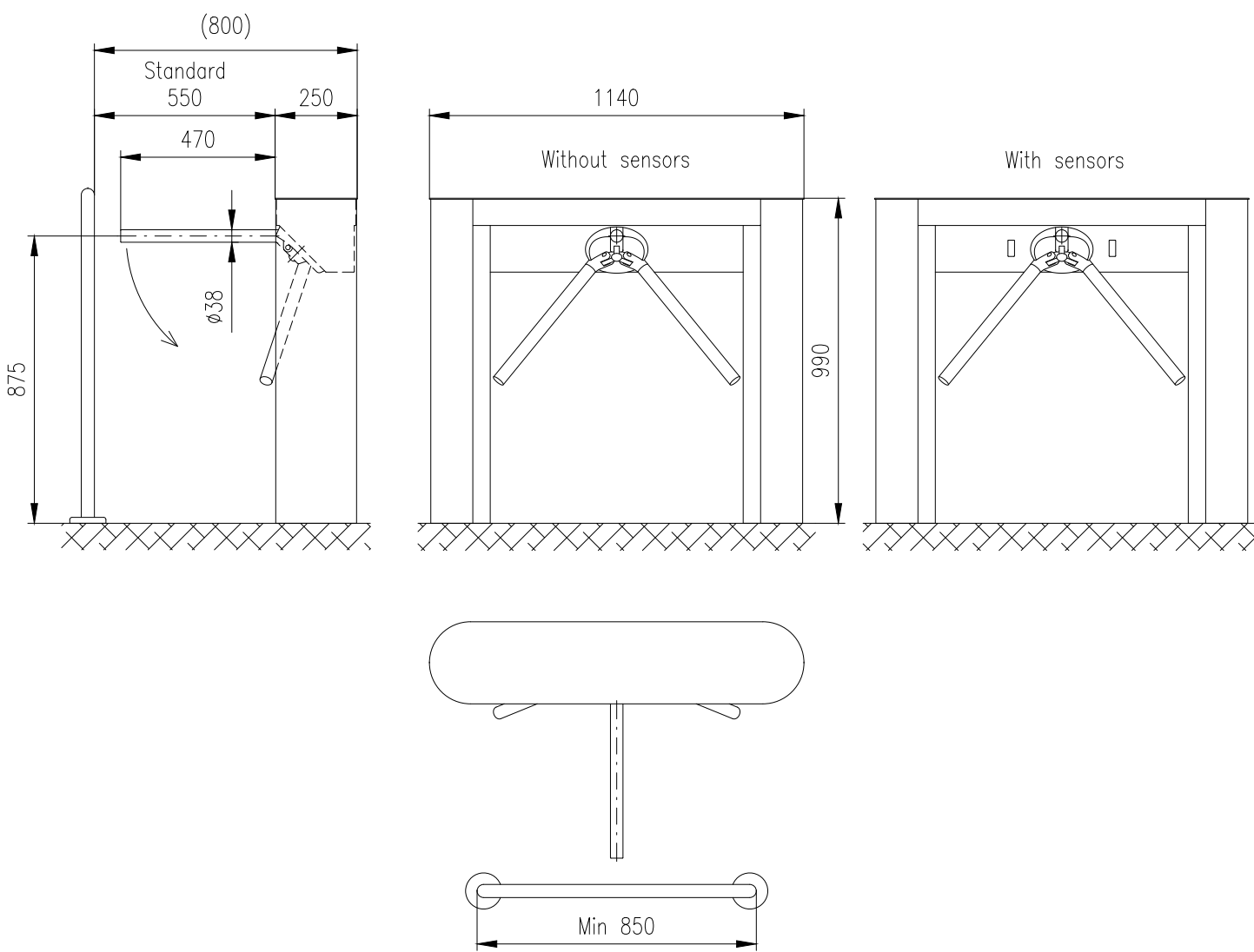
Turnstile: BAR–One–G–DropArm
