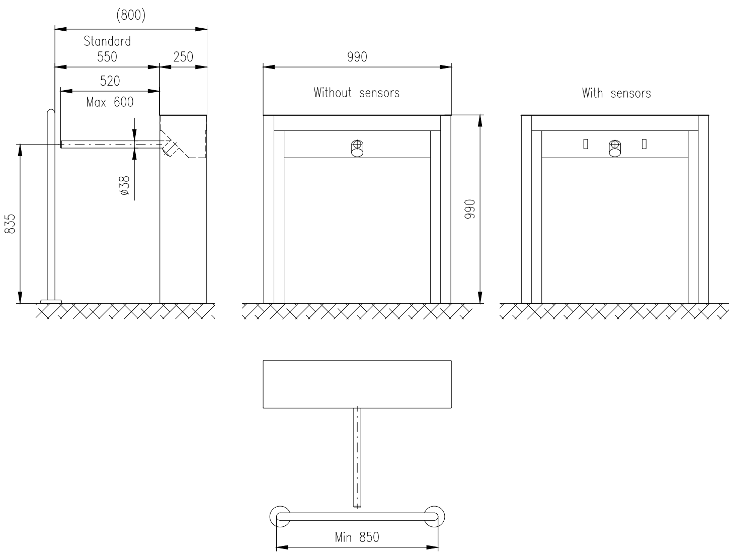
Turnstile: BAR–One–R–Unipod
