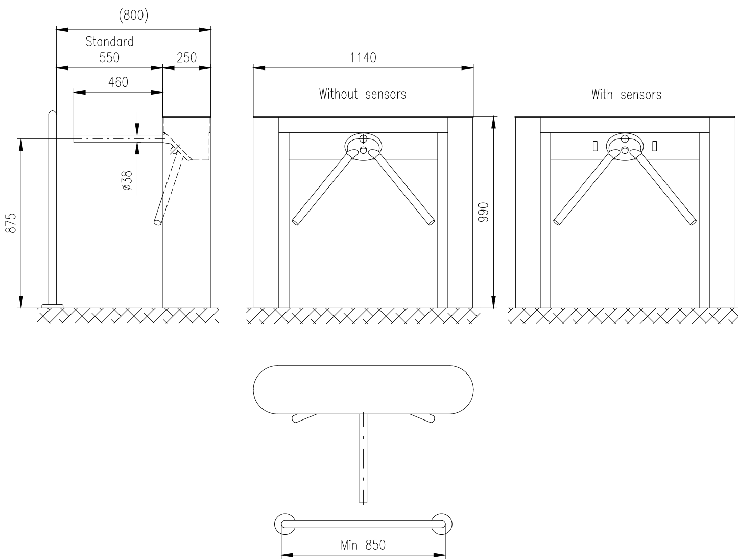
Turnstile: BAR–One–G–Tripod
