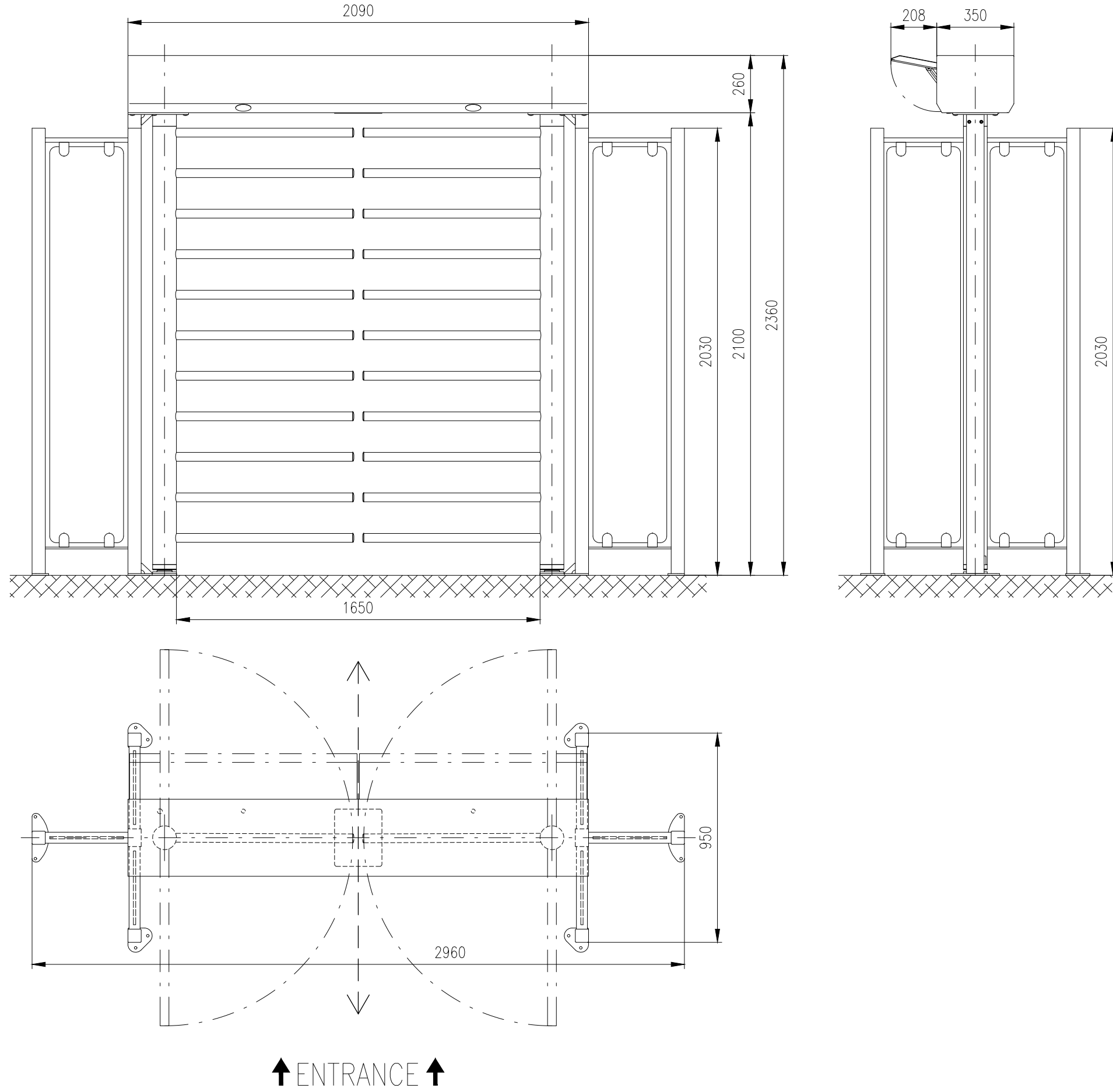
Motorized gate: GATE-ERA-DUO-GS-U (1650)
