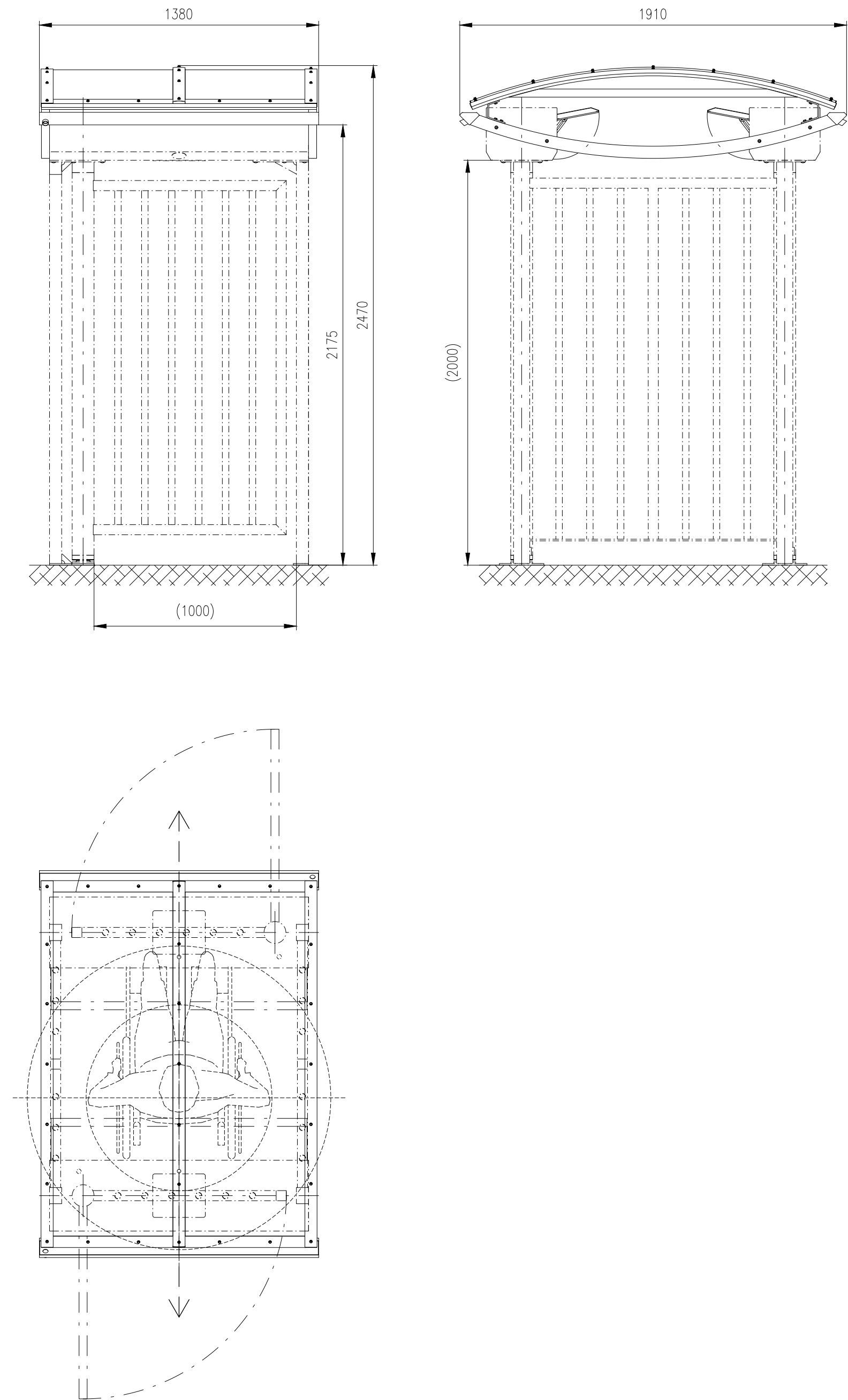
Roof for turnstile: GATE-INTERLOCK (1000)
