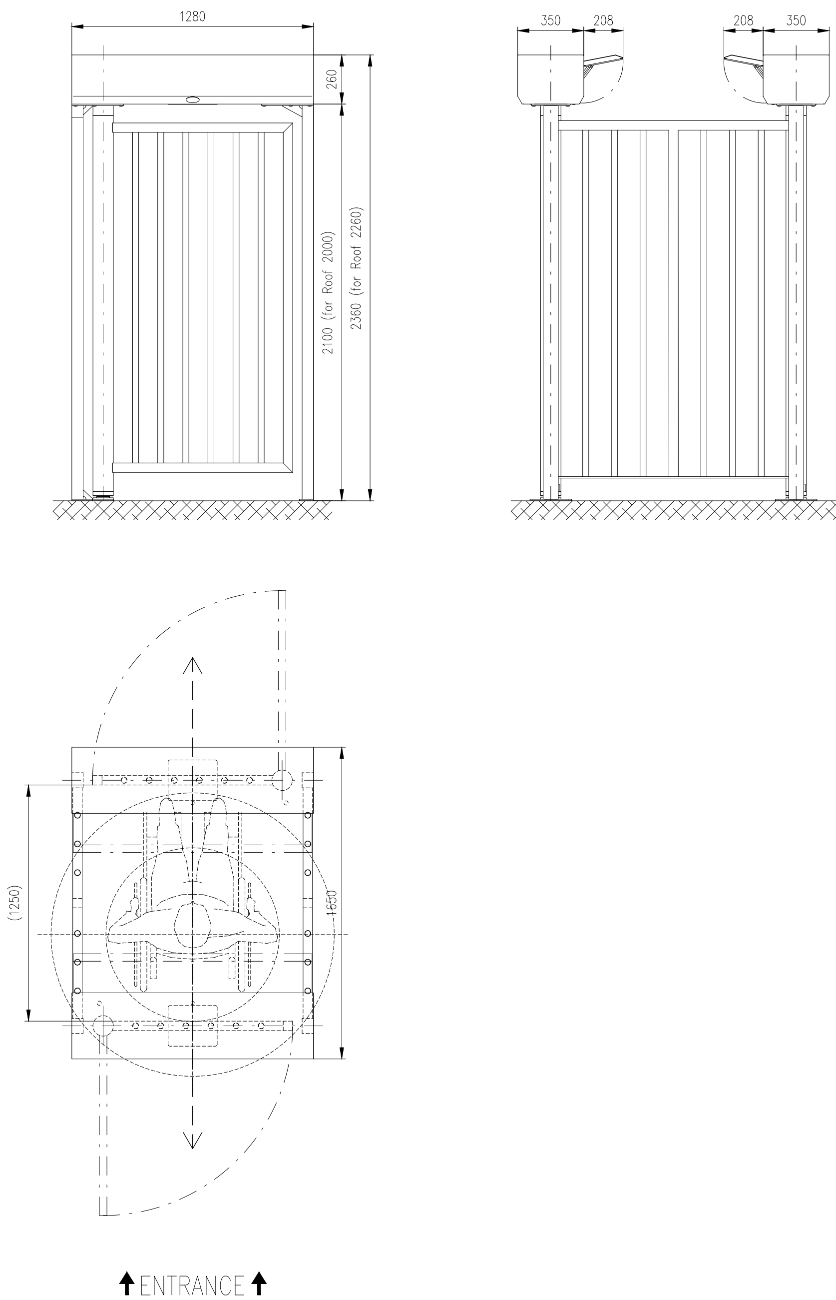
Motorized gate: GATE–INTERLOCK (1000)
