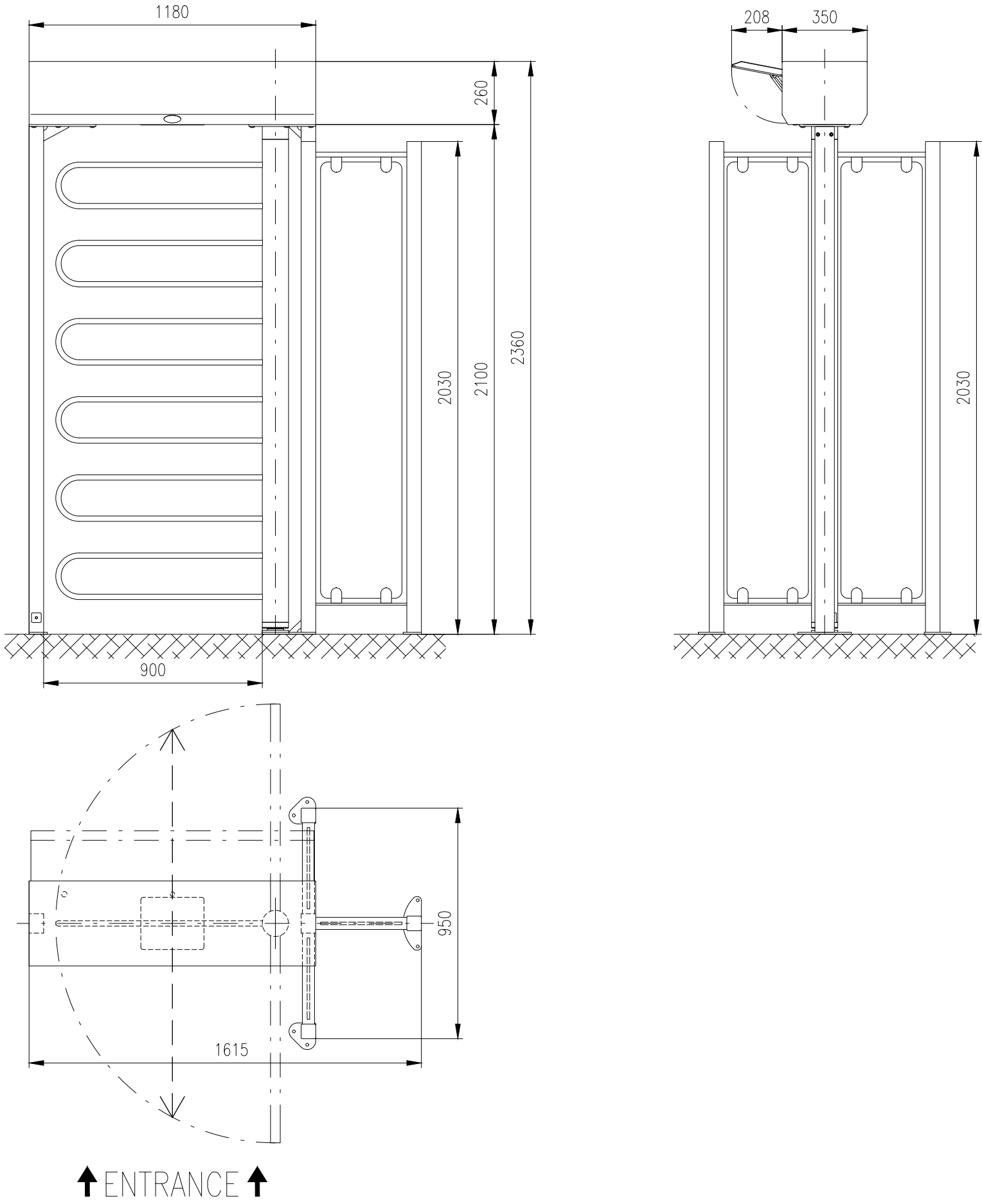
Motorized gate: GATE-ERA-GS-U (900)
