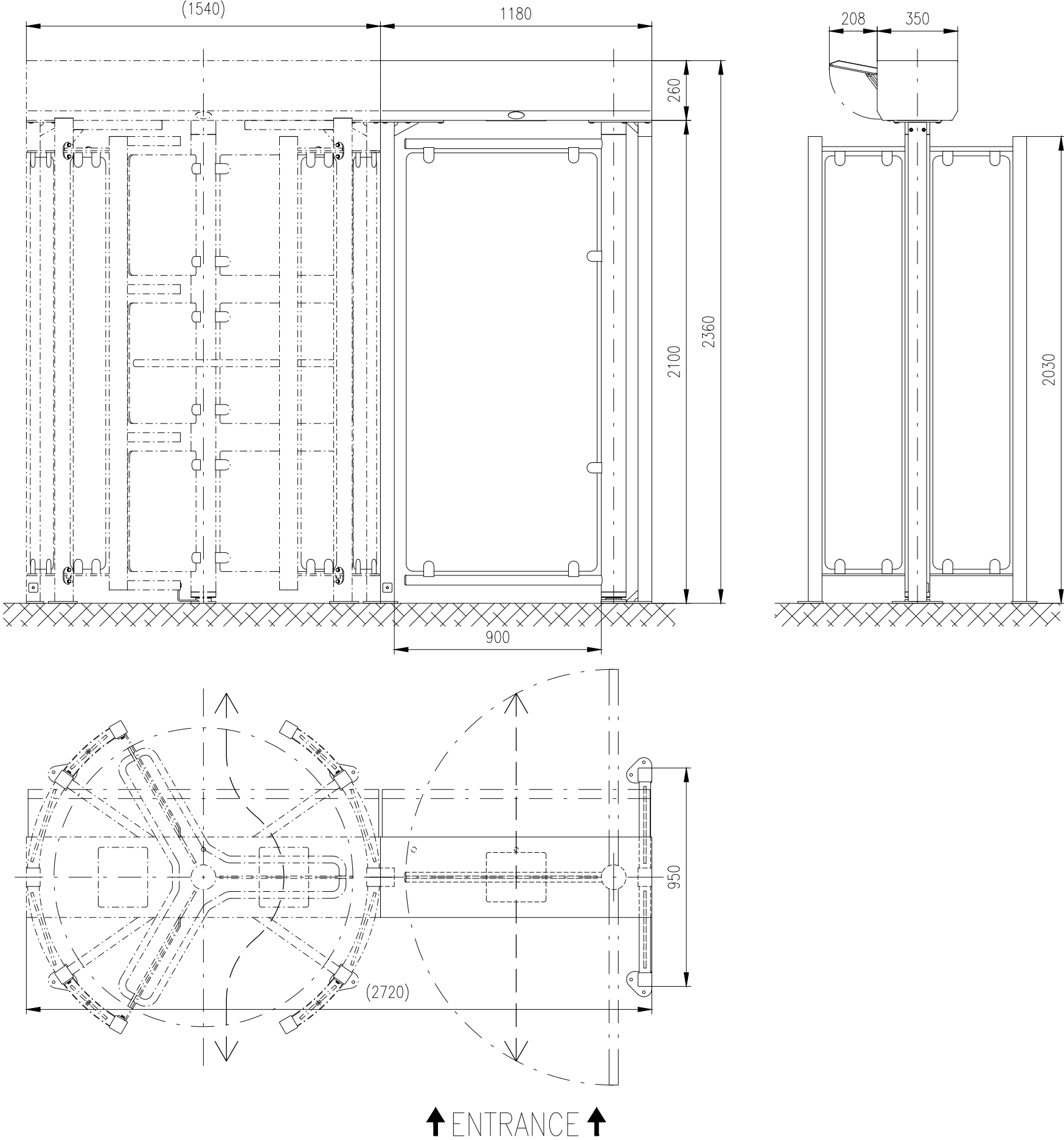
Motorized gate: GATE-ERA-GS-G (900)
