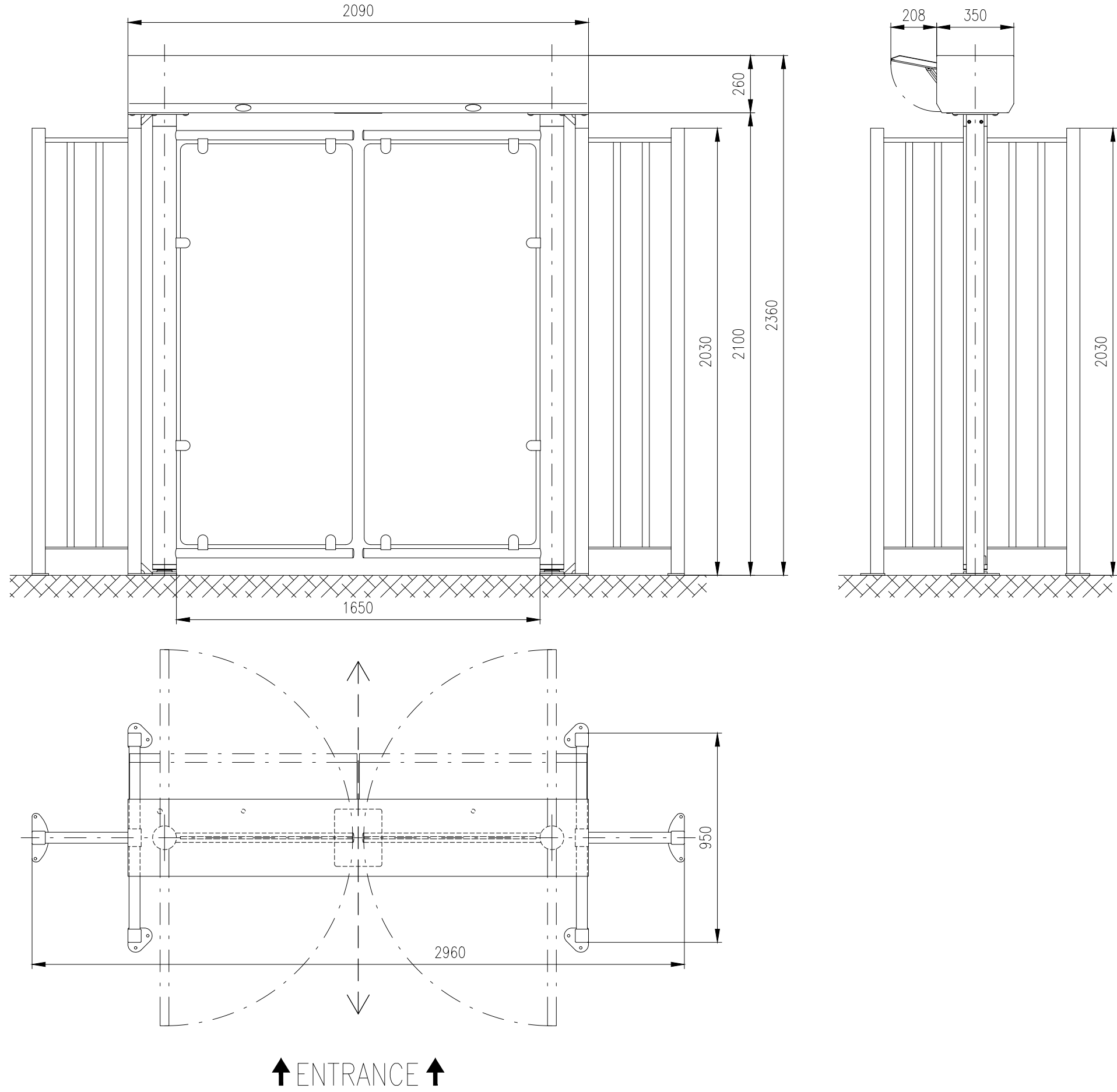
Motorized gate: GATE-ERA-DUO-GS-G (1650)
