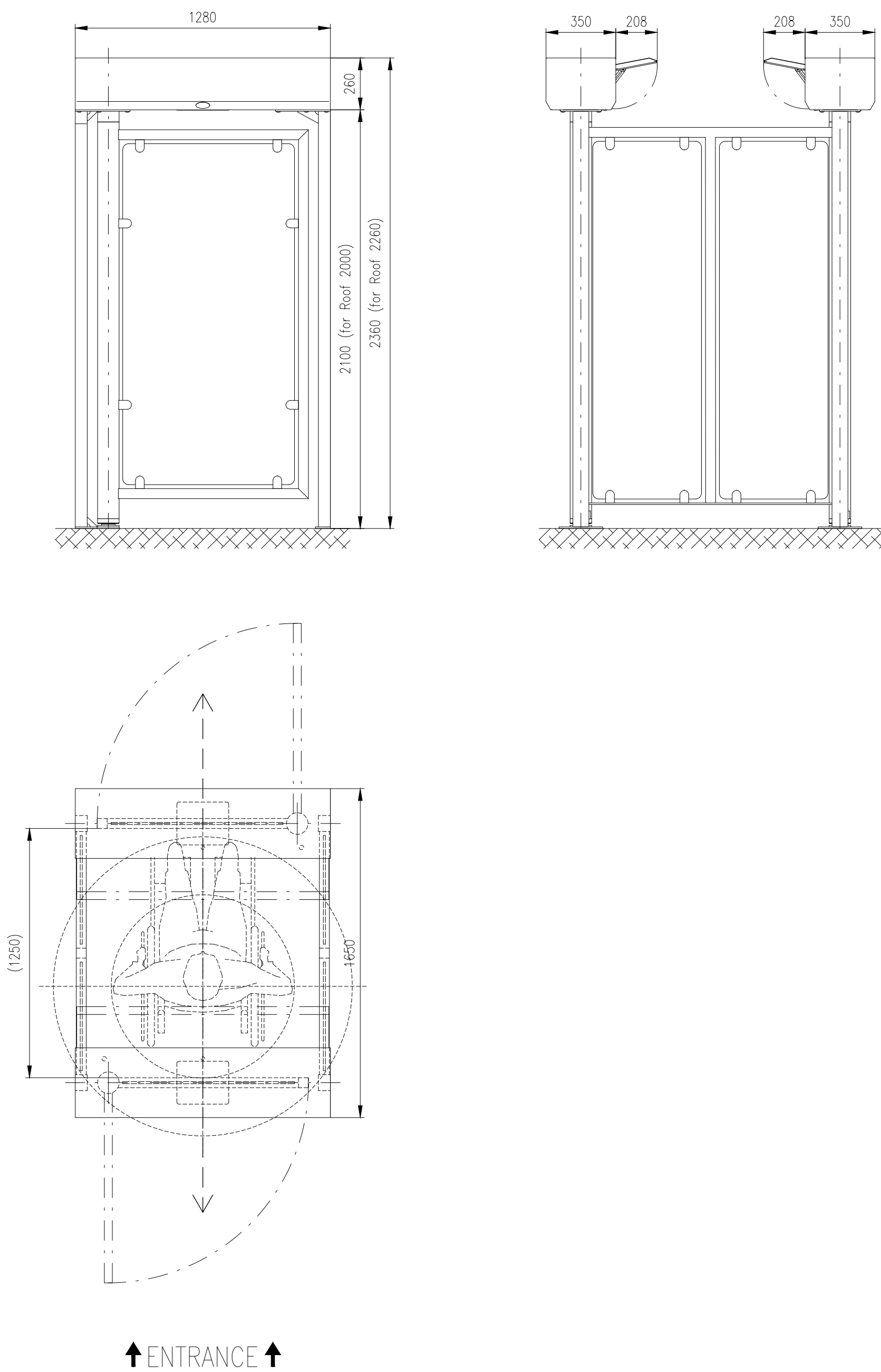
Motorized gate: GATE–INTERLOCK–GS–G (1000)
