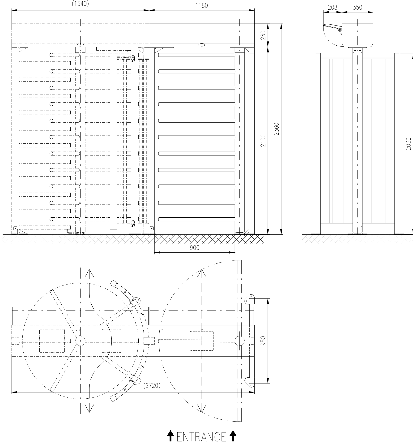
Motorized gate: GATE-ERA-U (900)
