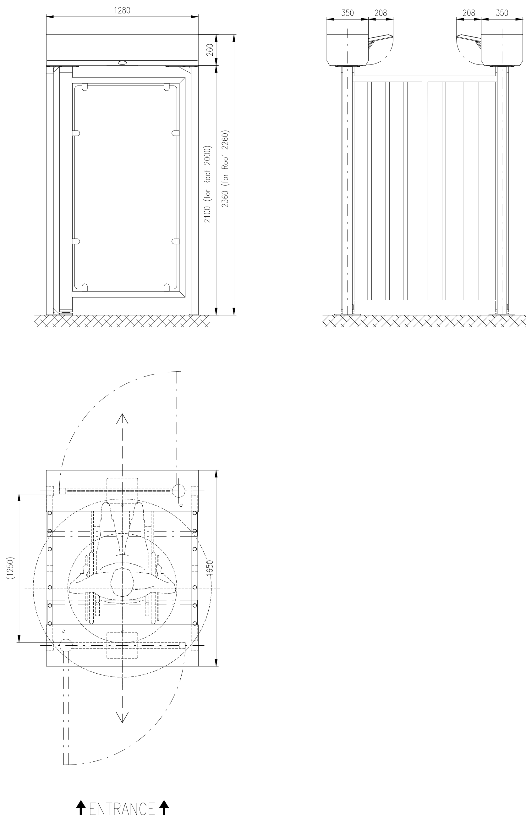
Motorized gate: GATE–INTERLOCK–G (1000)
