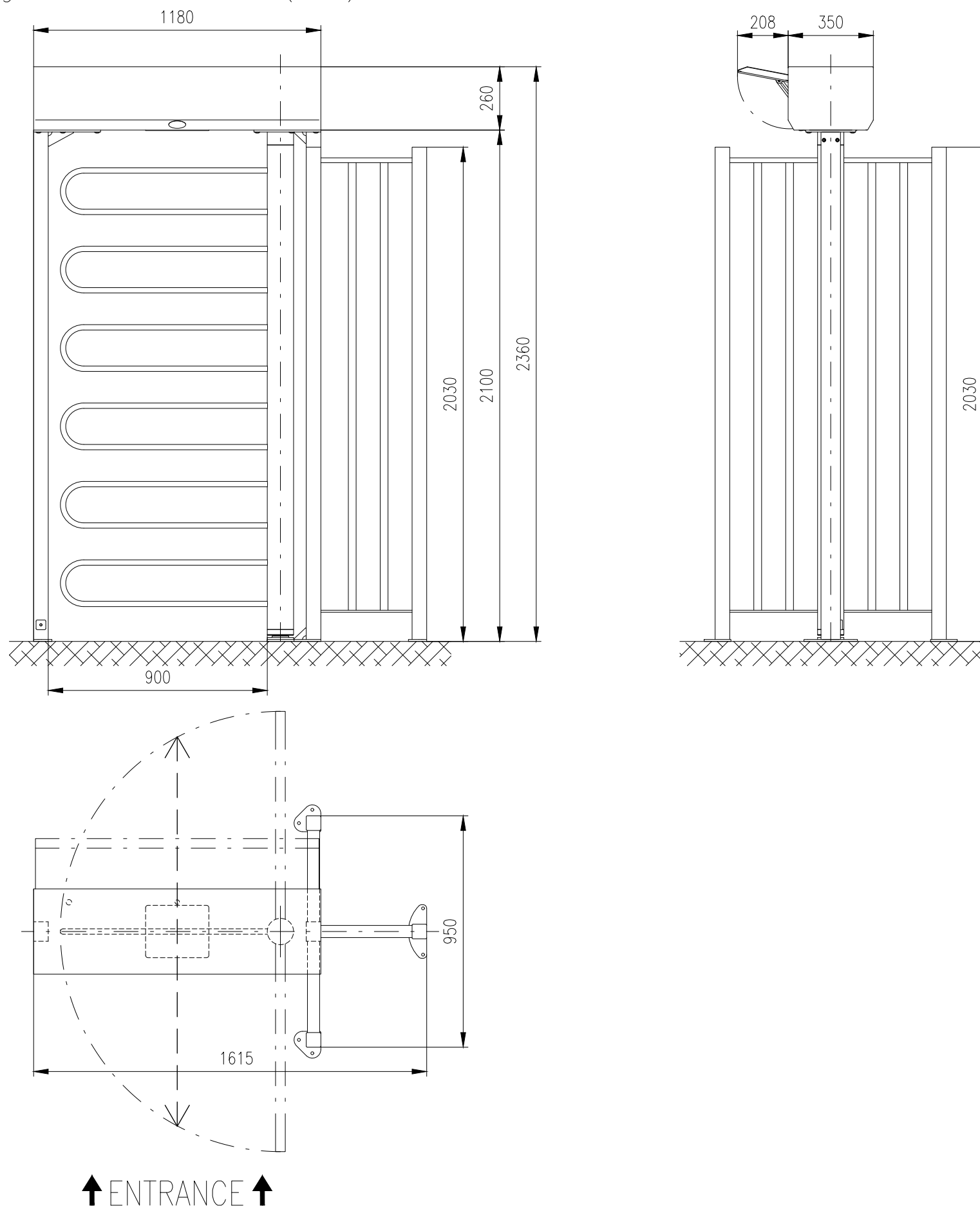
Motorized gate: GATE-ERA-U (900)
