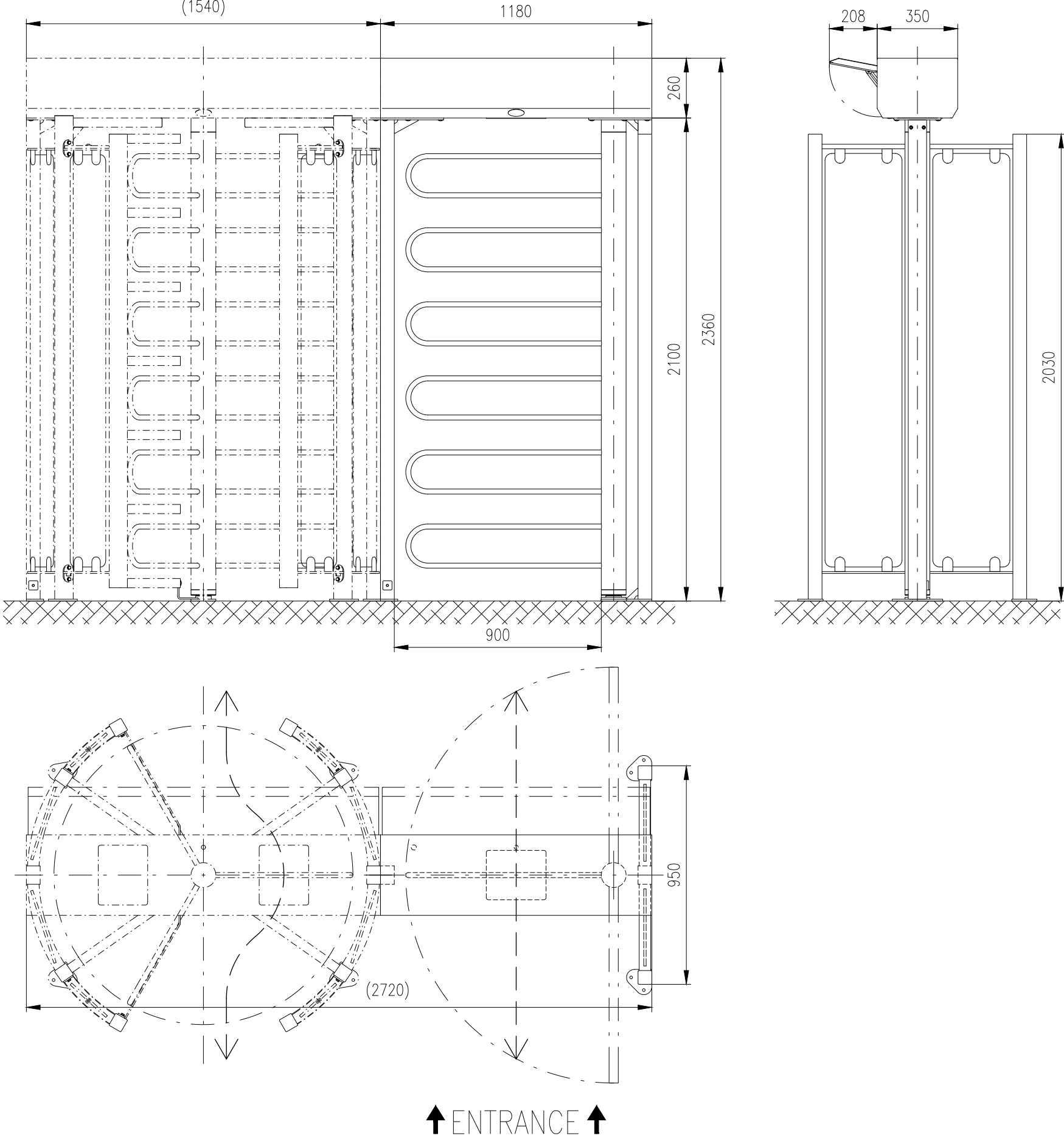
Motorized gate: GATE-ERA-GS-U (900)
