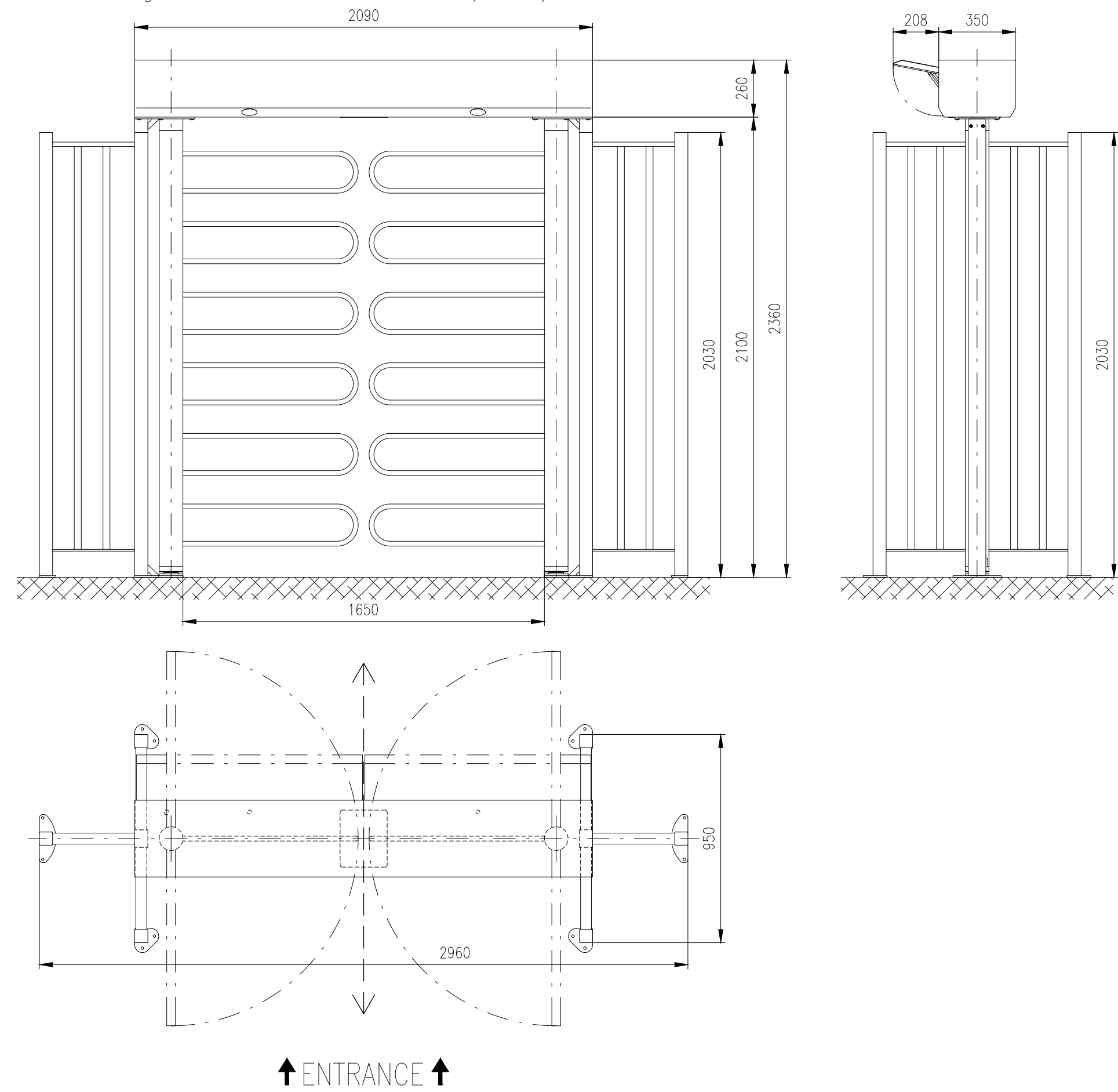
Motorized gate: GATE-ERA-DUO-U (1650)
