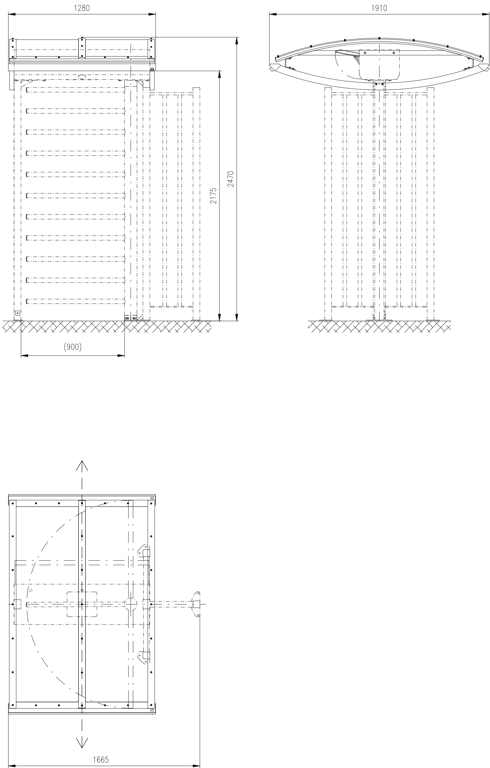
Roof for turnstile: GATE-ERA (900)
