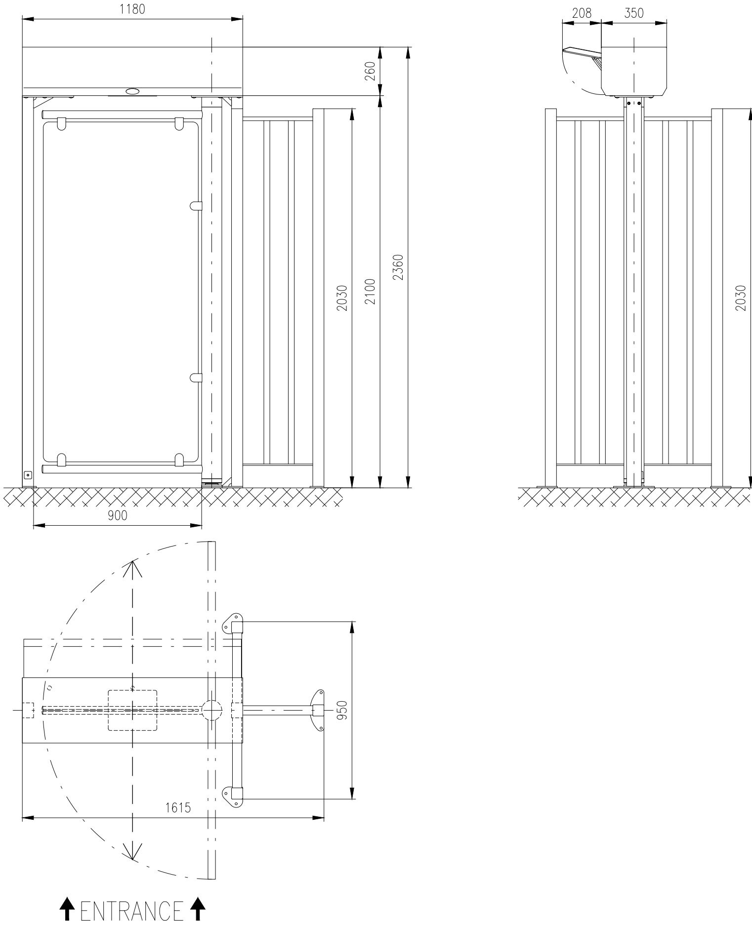
Motorized gate: GATE-ERA-GS-G (900)
