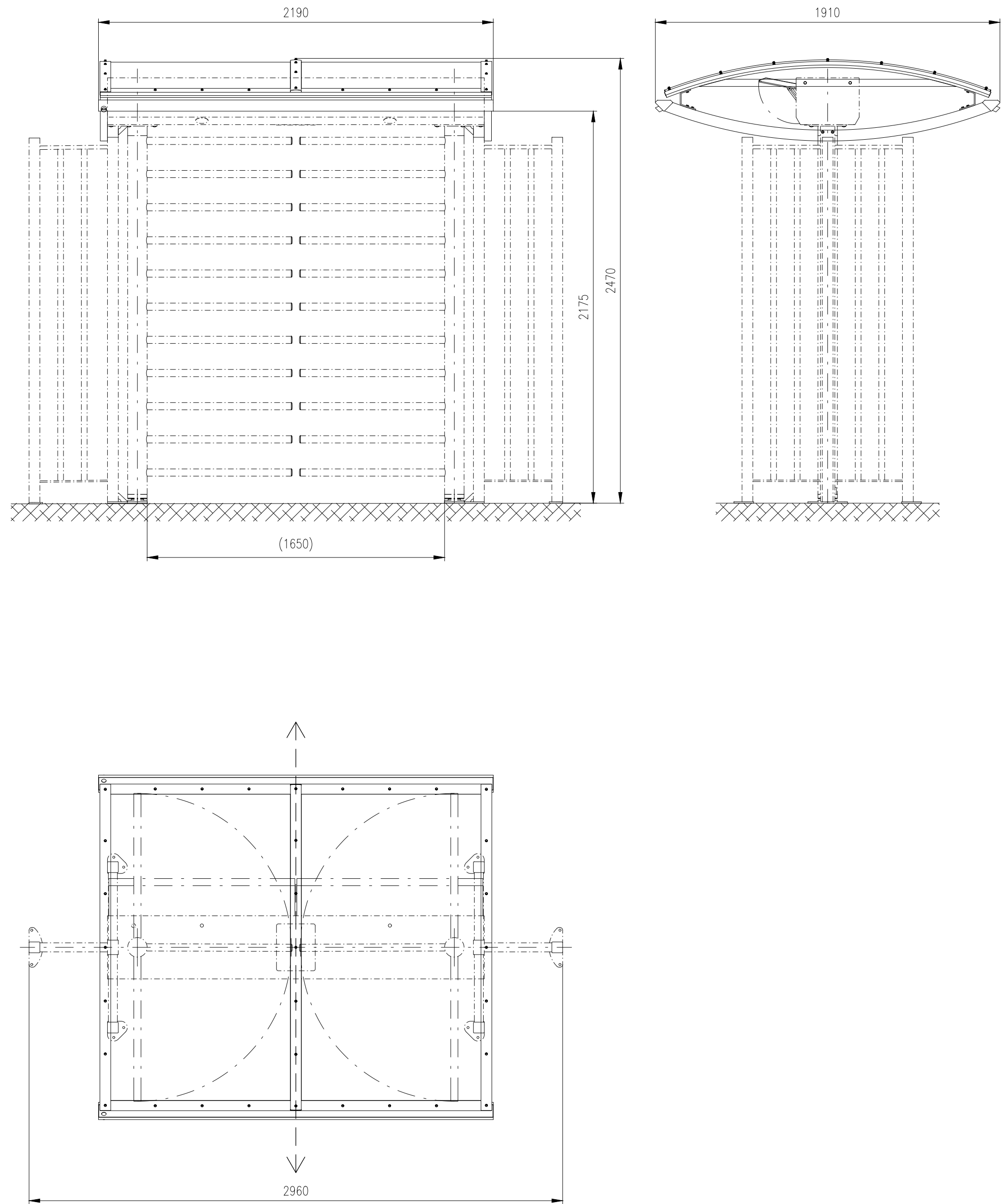
Roof for turnstile: GATE-ERA-DUO (1650)
