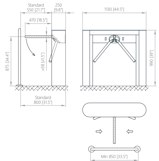
BAR One-G Tripod DropArm
