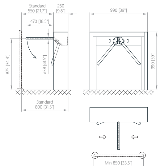
BAR One-R Tripod DropArm
